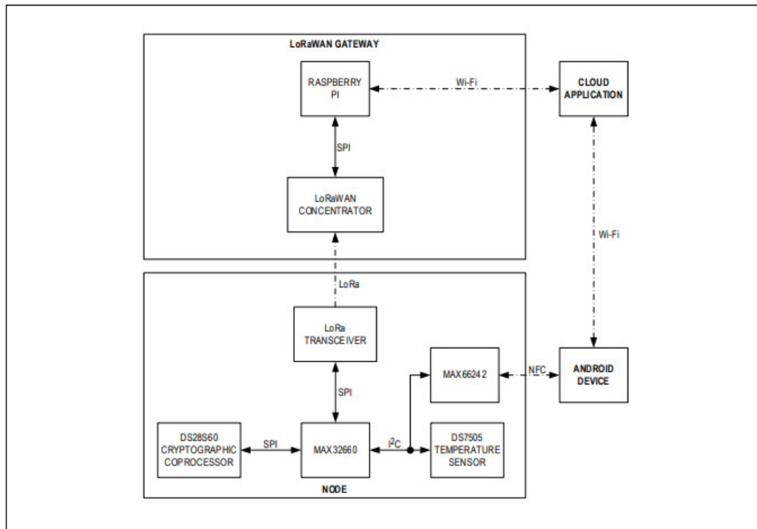
Figure 2. High-Level Block Diagram of the MAXREFDES9001
