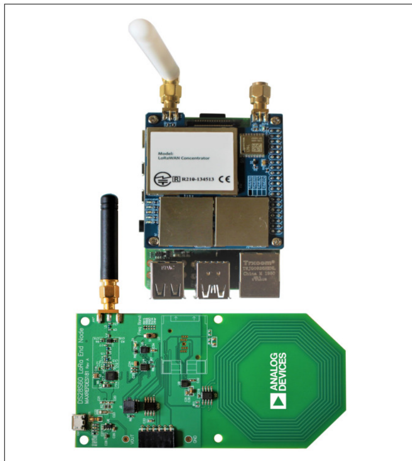
Figure 1. MAXREFDES9001 Hardware
