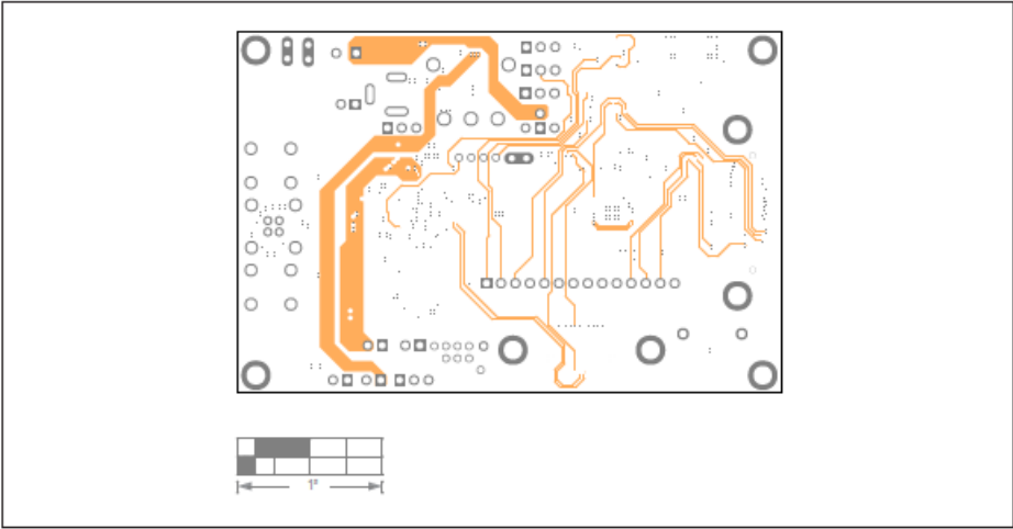
MAX96752 EV Kit PCB Layout—Internal5
