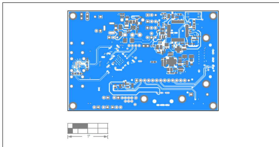
MAX96752 EV Kit PCB Layout—Bottom
