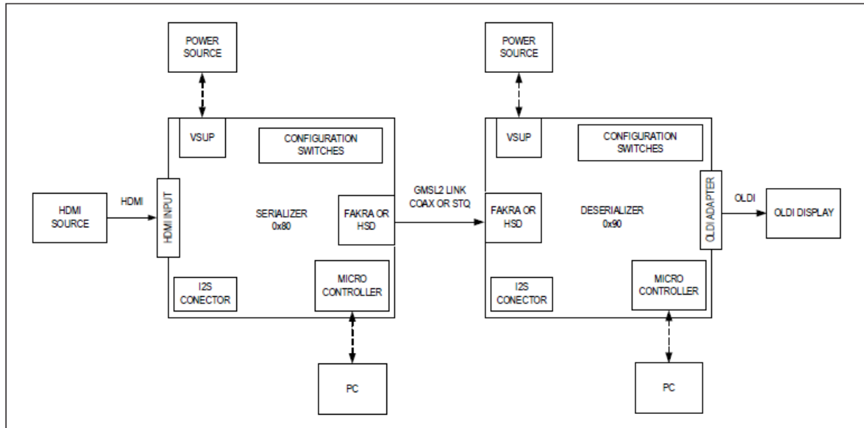
Figure 2. Typical GMSL System Evaluation Setup Block Diagram
