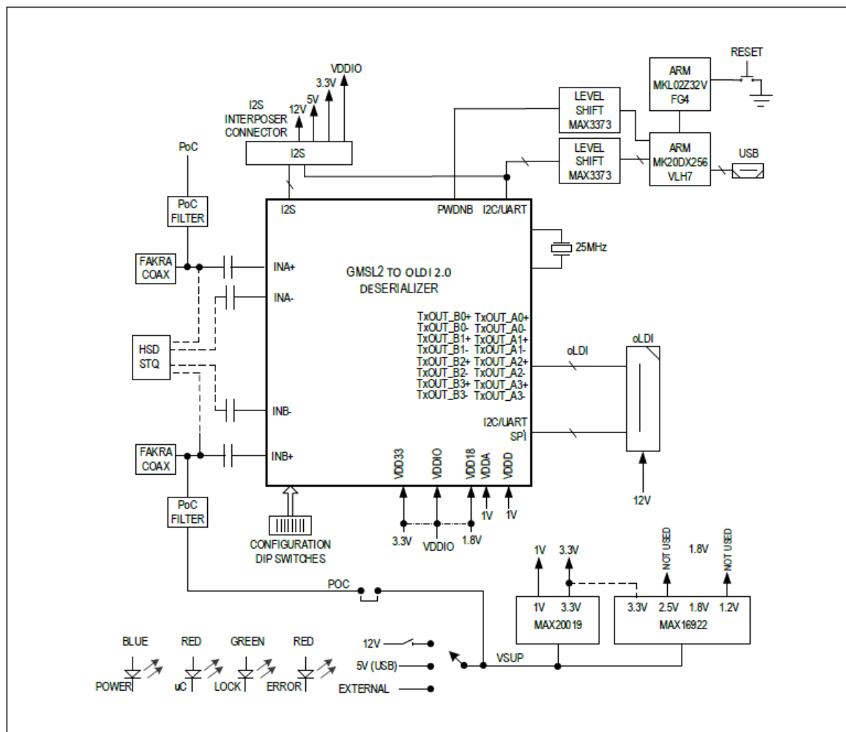
Figure 1. Deserializer Evaluation Board Block Diagram
