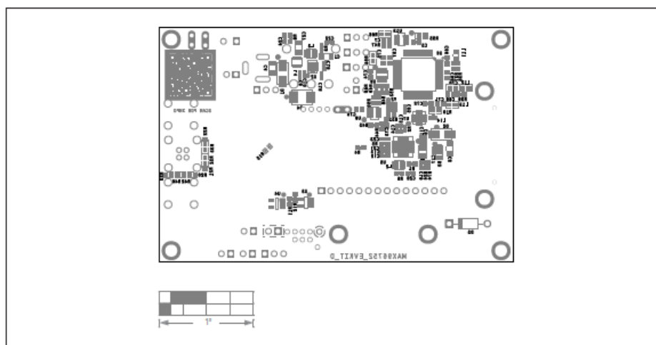
MAX96752 EV Kit Component Placement Guide—Bottom Silkscreen
