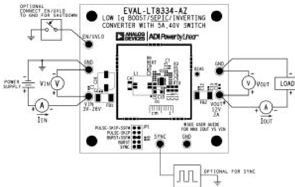
Figure 1. Proper Equipment Setup for EVAL-LT8334-AZ
