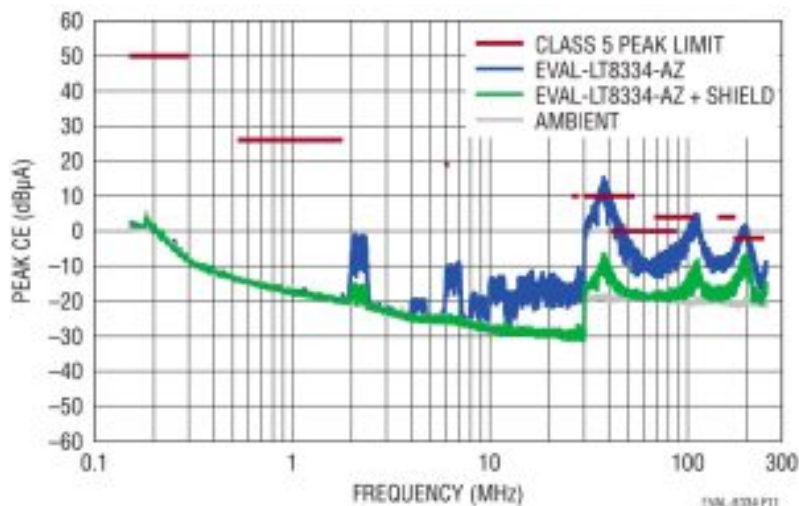
Figure 11. EVAL-LT8334-AZ CISPR25 Current Conducted EMI Peak Performance with 12VIN to 12VOUT at 2A, JP1 = BURST+SSFM
