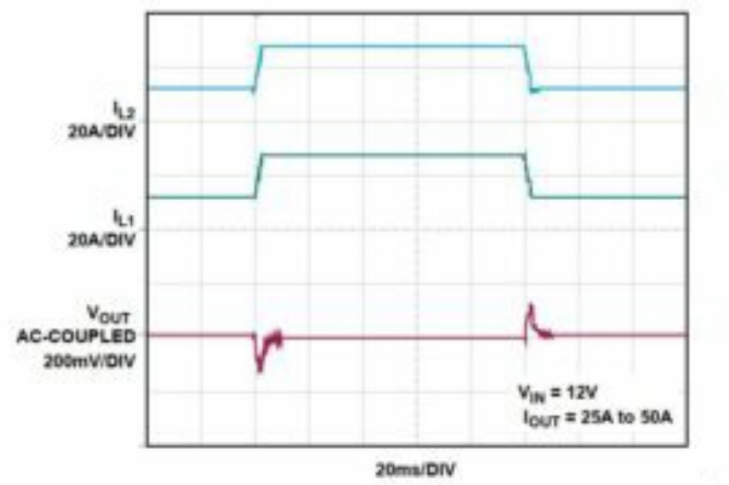
Figure 5. Load Transient Response at V_{IN} = 12V , 25A to 50A
