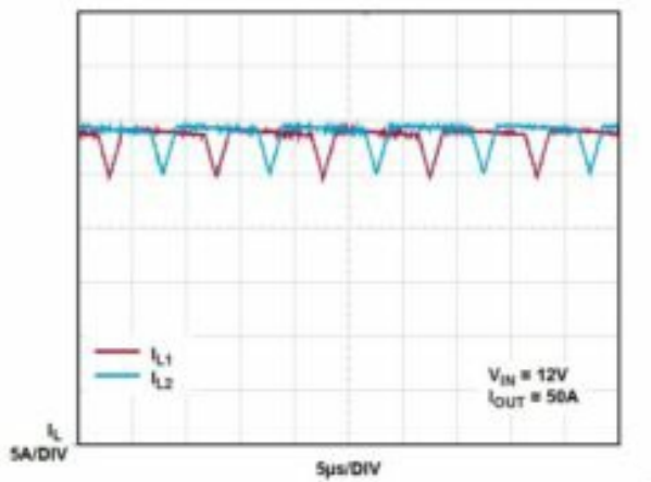
Figure 4. Inductor Current with 180° phasing at V_{IN} = 12V , I_{OUT} = 50A
