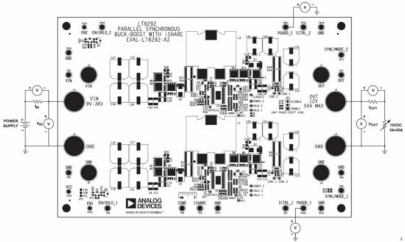
Figure 1. EVAL-LT8292-AZ Board Connections
