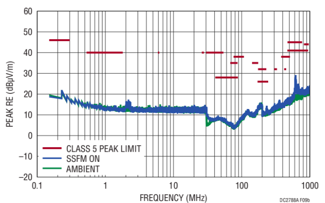
(b) CISPR25 Radiated EMI Performance
