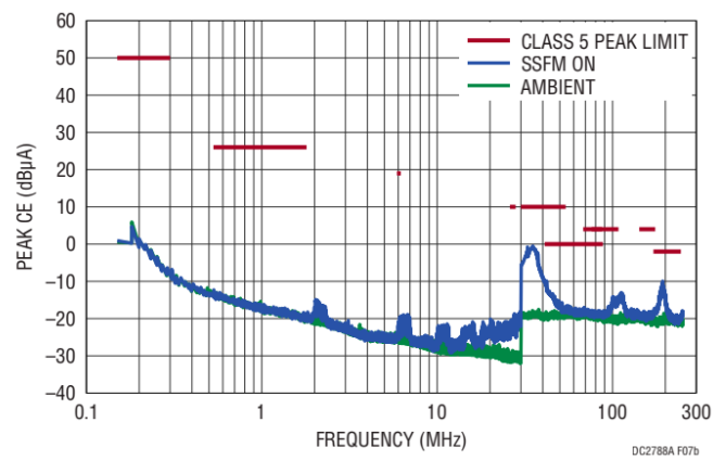
(b) CISPR25 Conducted EMI Performance Current Method
