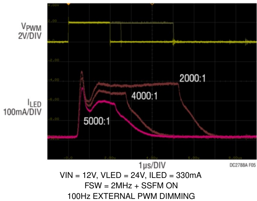
Figure 5. Up to 5000:1 PWM Dimming is Possible, Even with EMI Filters on DC2788A
