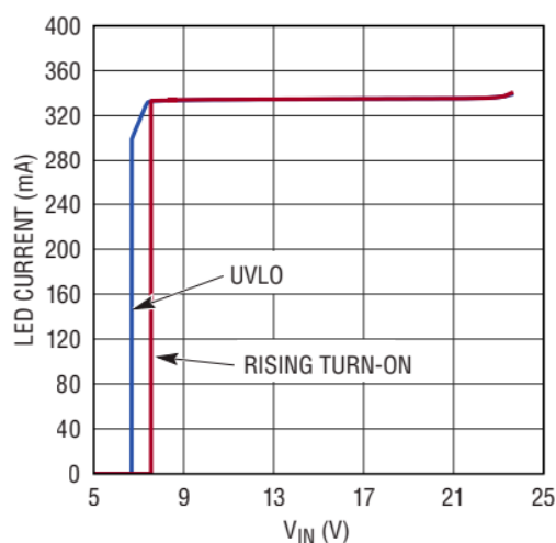
(b) LED Current vs Input Voltage
