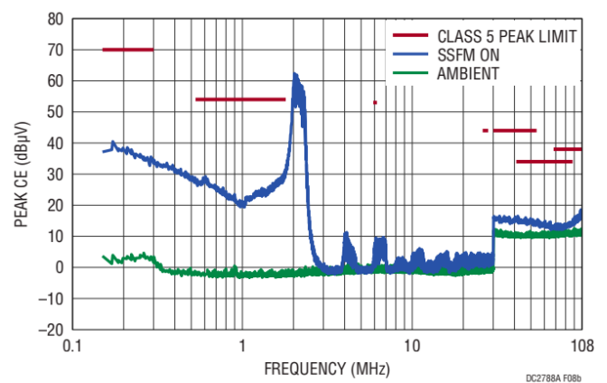
(b) CISPR25 Conducted EMI Performance Voltage Method
