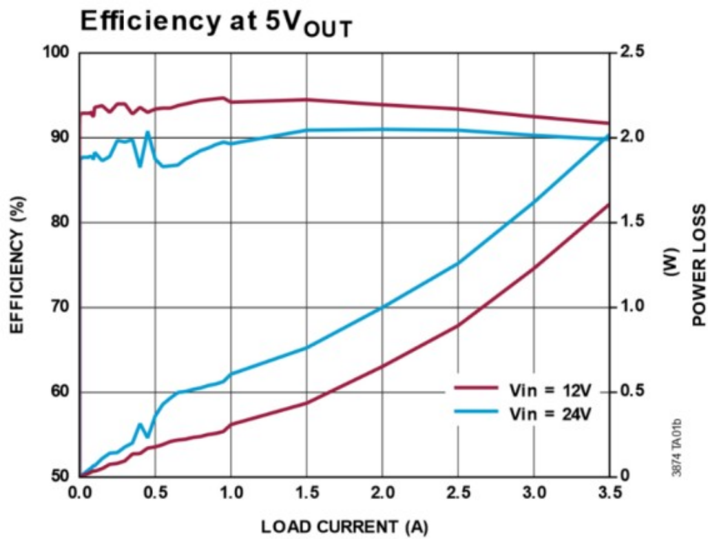
Figure 1. LT8641A Eval Circuit Efficiency vs. Load Current (2MHz Switching Frequency, Burst Mode)
