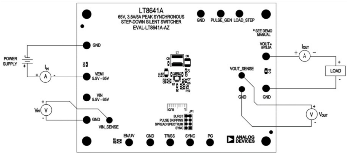
Figure 3. Proper Measurement Equipment Setup
