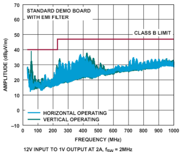
Figure 4. LT8622S Data Sheet Typical Application Circuit Noise Spectral Density (12V Input to 1.0V Output, f_{SW} =
