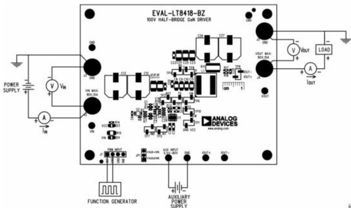
Figure 1. EVAL-LT8418-BZ Board Connections in Single-PWM-Input Control Mode
