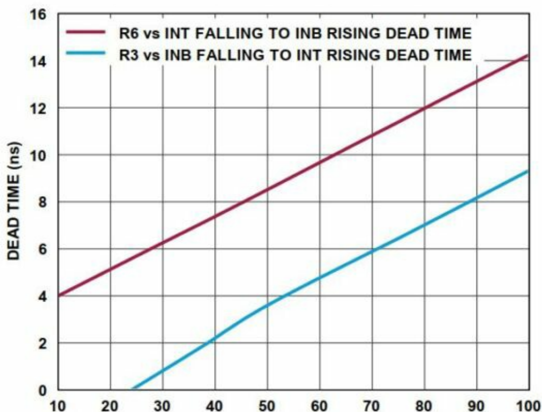
Figure 2. Dead Times vs. Resistor Values
