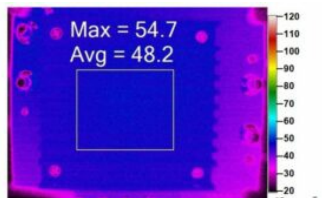
Figure 16. Thermal Image of Bottom Layer at 24V OUT , 10A I OUT , 1MHz (with Heat Sink, Thermal Values are on Heat Sink)
