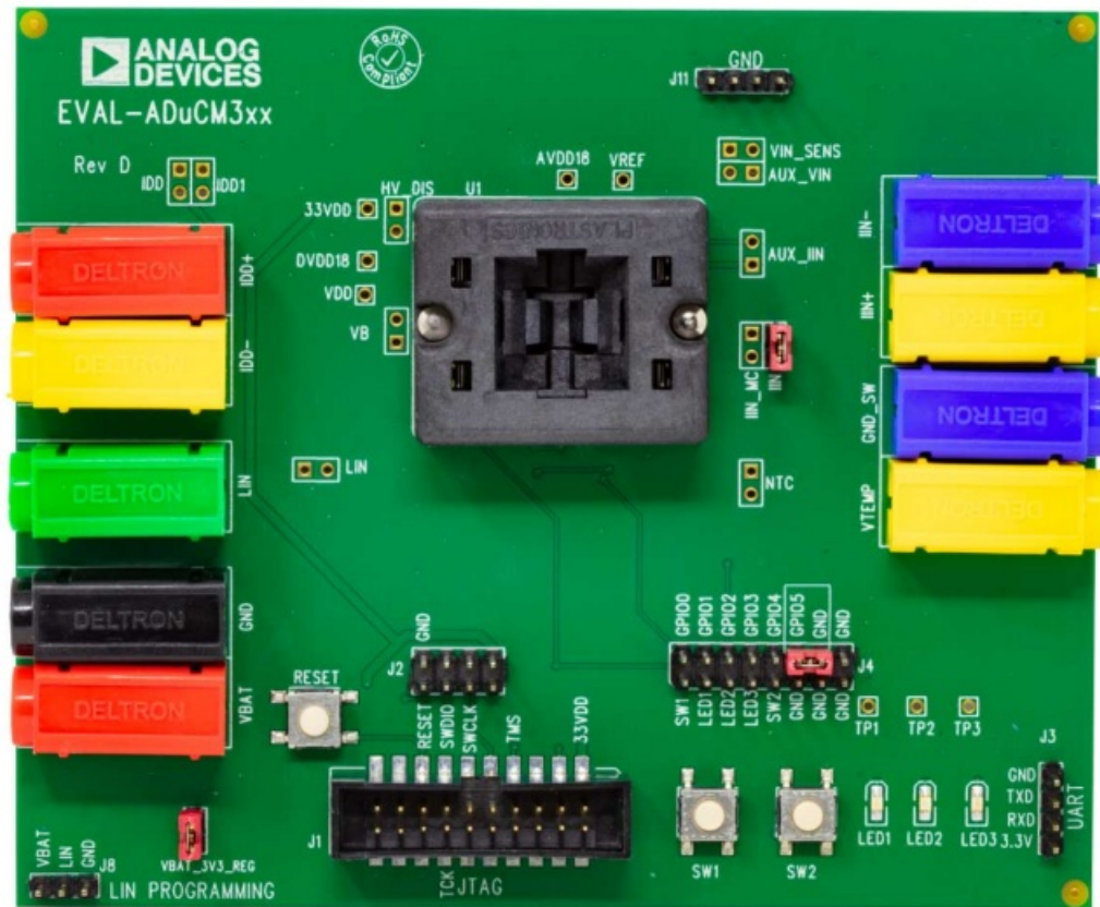
Figure 1. EVAL-ADuCM342EBZ Socketed Evaluation Board Setup
