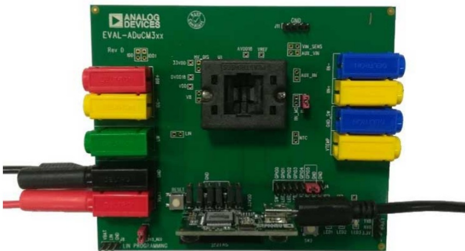
Figure 4. Mini-Link Debugger/Programmer Connection
