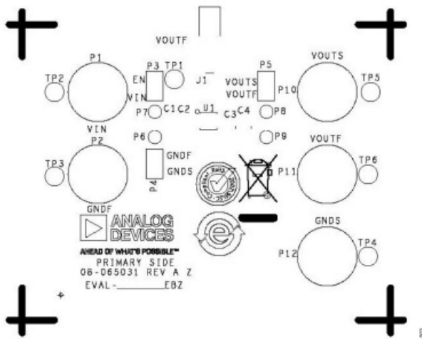
Figure 3. EVAL-ADR3625EBZ Silkscreen
