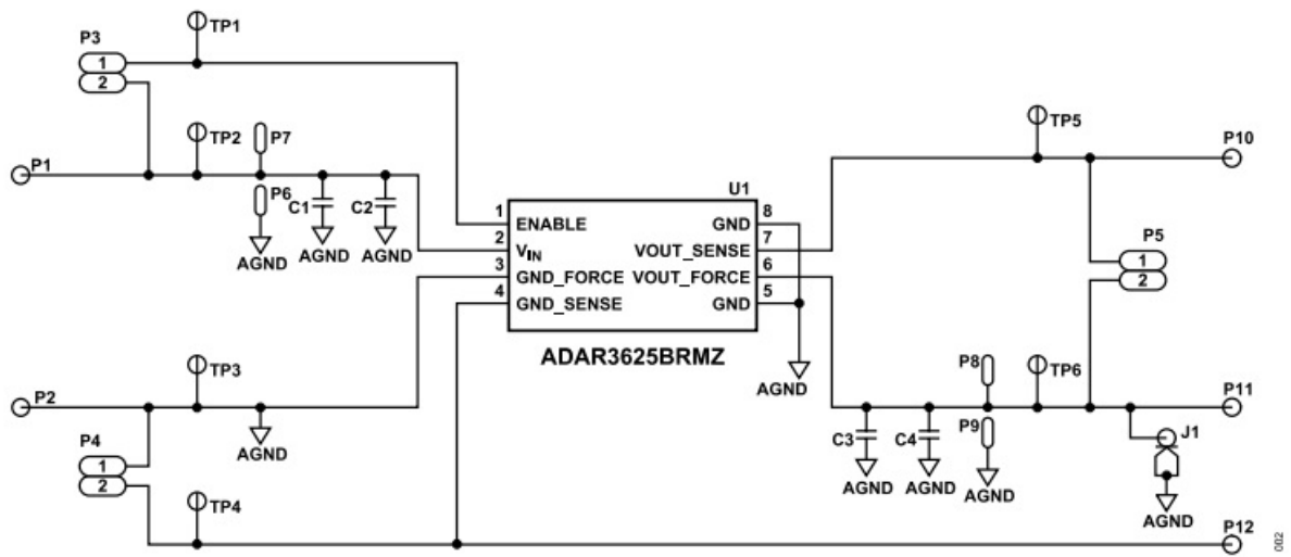
Figure 2. EVAL-ADR3625EBZ Evaluation Board Schematic
