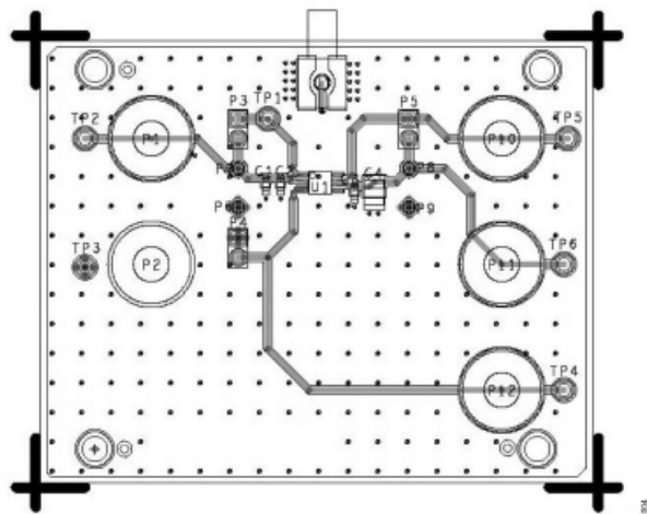
Figure 4. EVAL-ADR3625EBZ Top Layer
