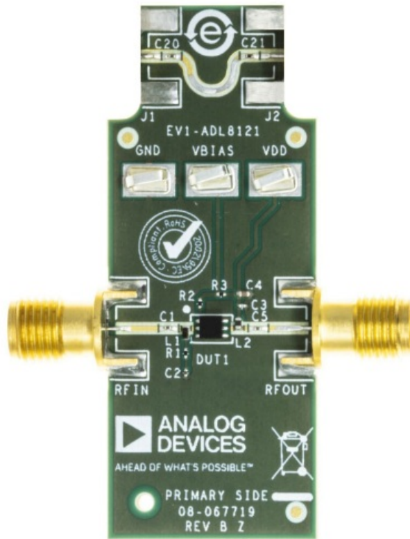
Figure 1. ADL8121-EVALZ Primary Side
