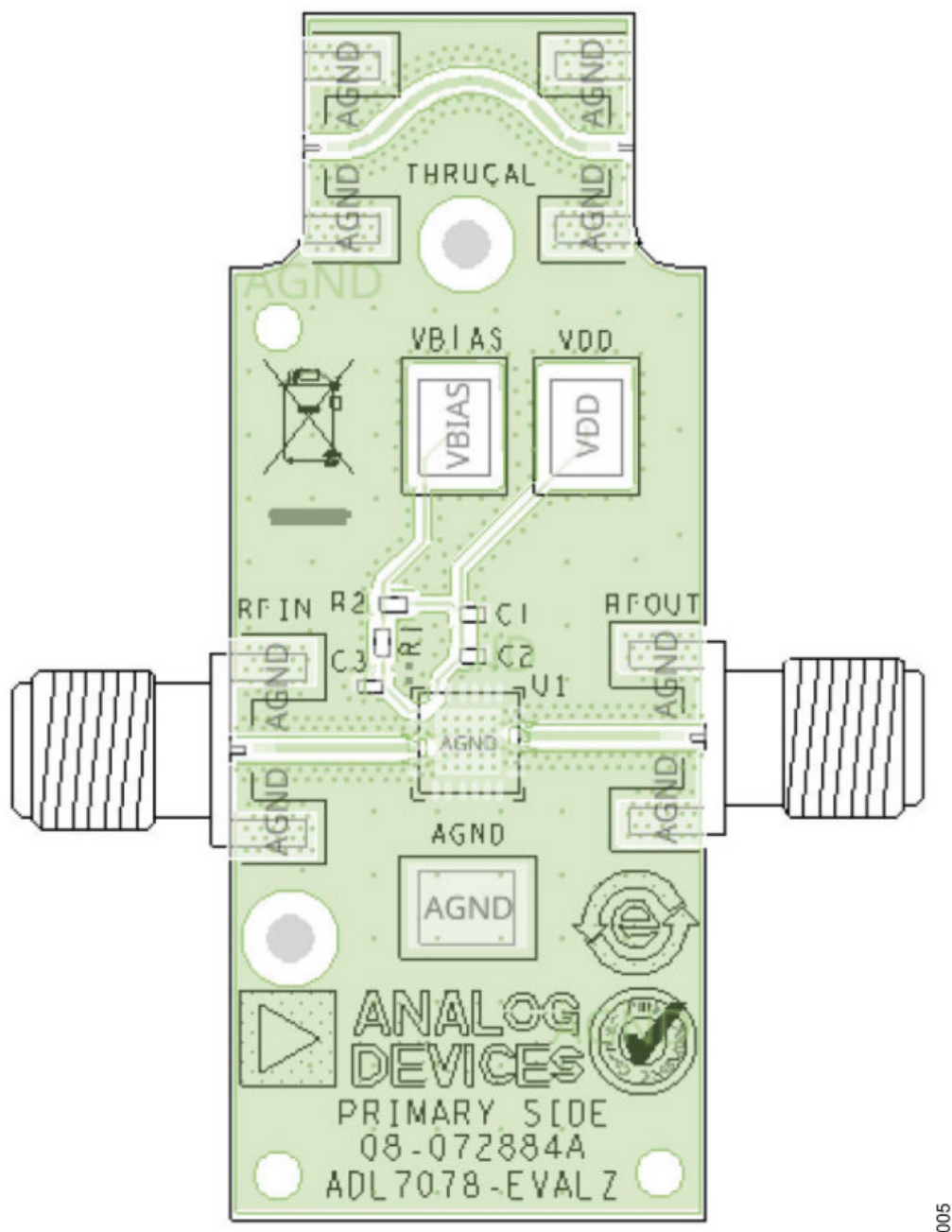
Figure 6. ADL7078-EVALZ Assembly Drawing (J1 and J2 Are Not Installed)
