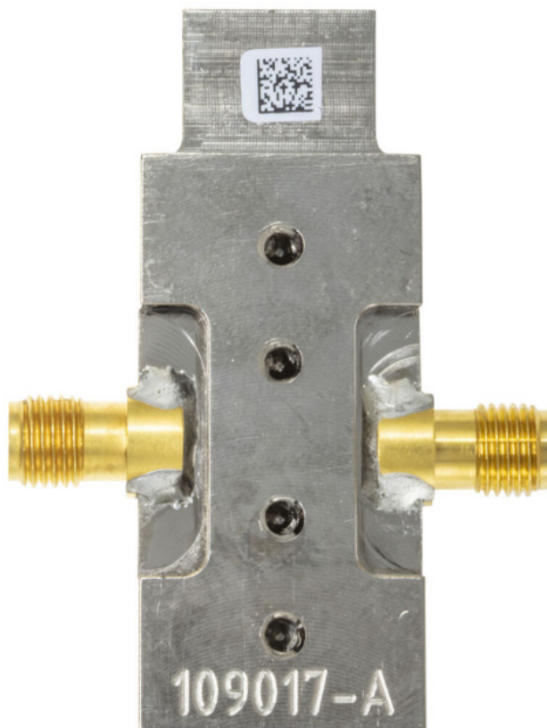
Figure 2. ADL7078-EVALZ Secondary Side
