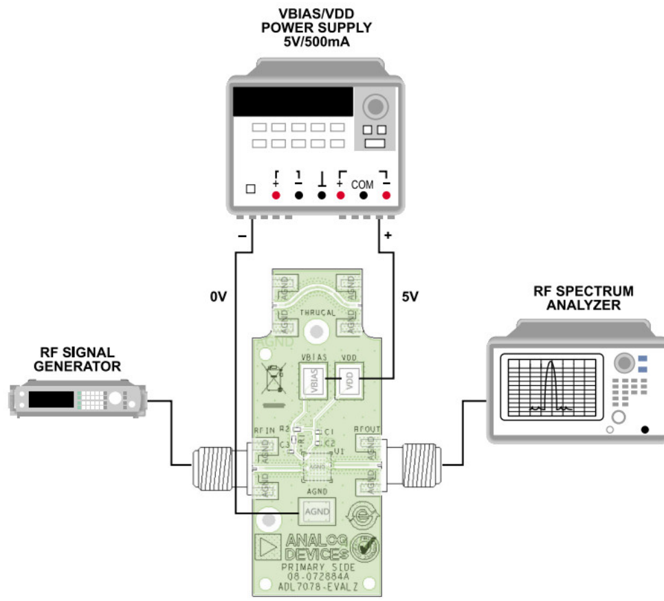
Figure 3. Operating Block Diagram of ADL7078-EVALZ
