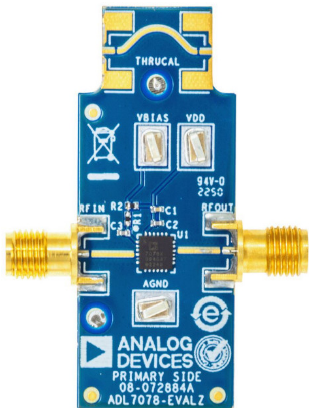
Figure 1. ADL7078-EVALZ Primary Side
