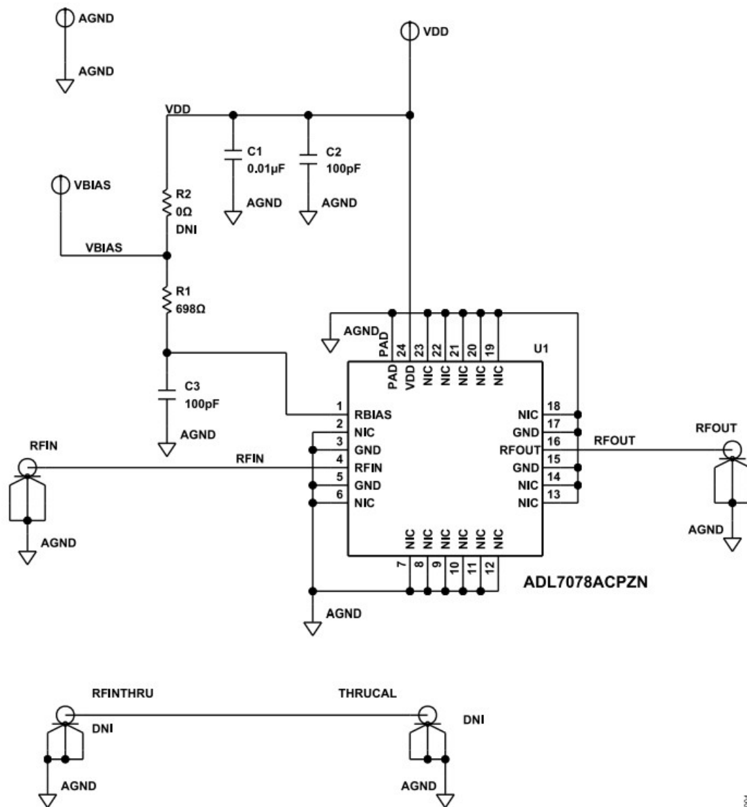
Figure 5. ADL7078-EVALZ Schematic
