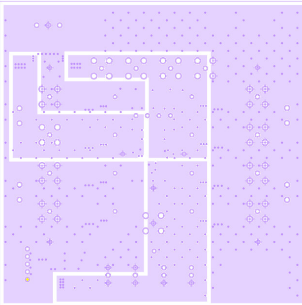
Figure 6. EVAL-ADG1412LEBZ Layer 3
