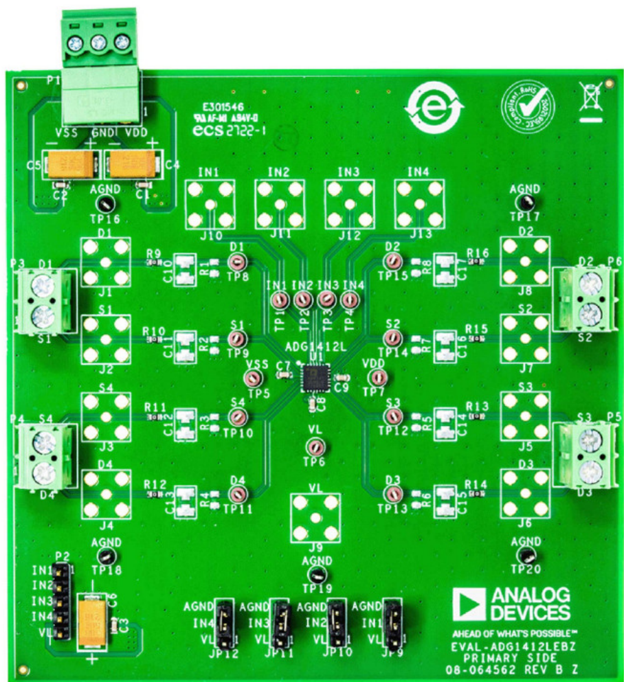
Figure 1. EVAL-ADG1412LEBZ Photograph
