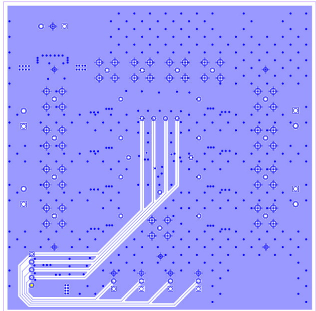
Figure 7. EVAL-ADG1412LEBZ Bottom Layer
