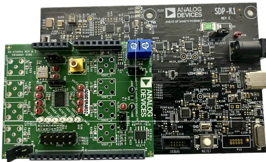
Figure 1. Evaluation Board Connected to the SDP-K1 Controller Board (EVAL-AD5675RARDZ or EVAL-AD5676R2ARDZ)
