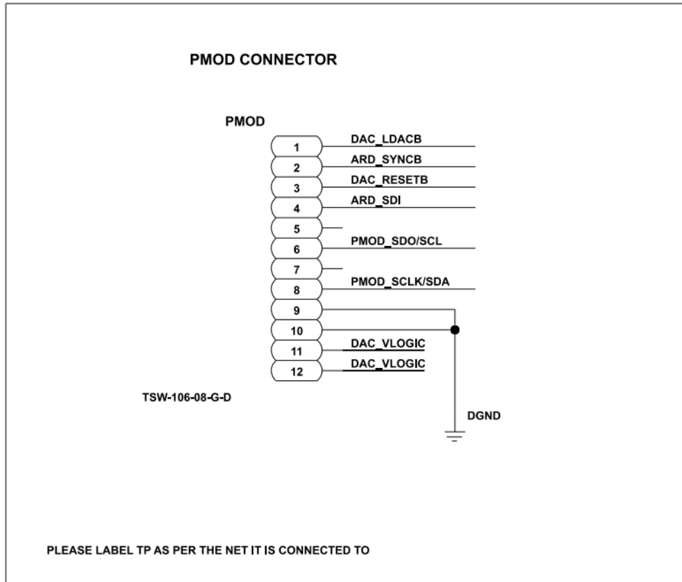
Figure 11. NanoDAC+ Evaluation Board Schematic Diagram, PMOD Connection
