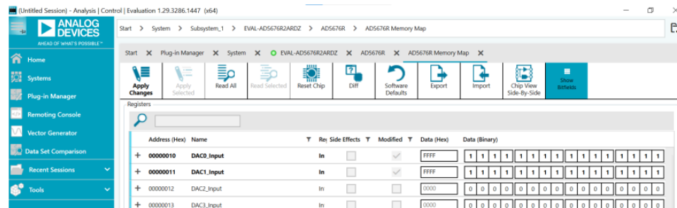
Figure 7. AD5675R or AD5676R Memory Map with Pending Changes in DAC0_Input_Register
