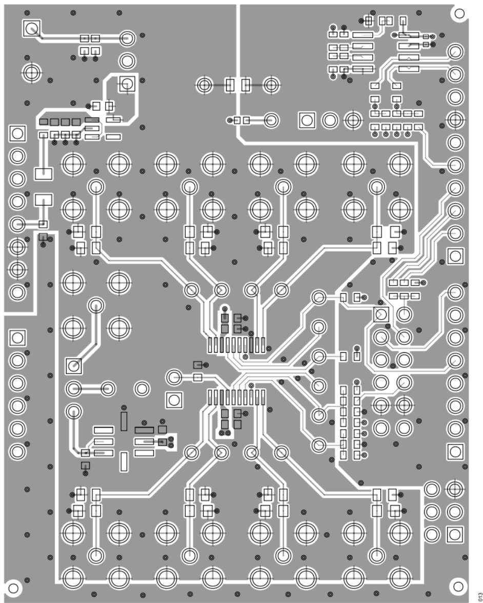
Figure 13. NanoDAC+ Evaluation Board, Top Side Routing
