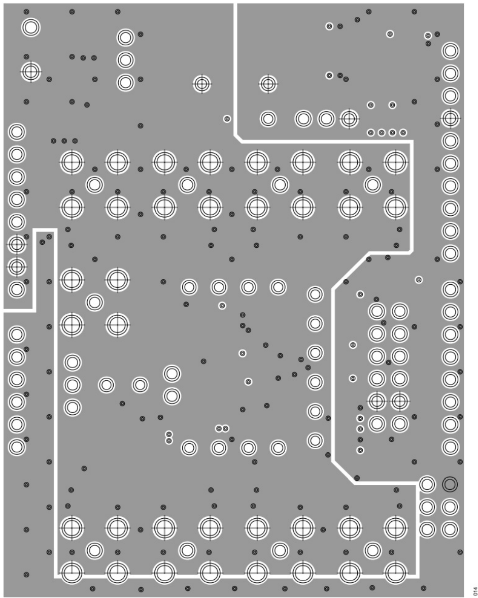
Figure 14. NanoDAC+ Evaluation Board, Bottom Side Routing
