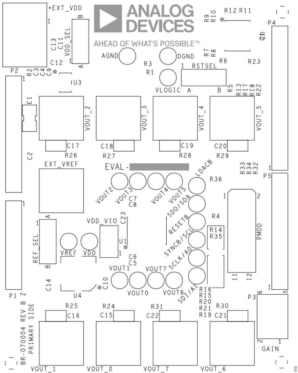
Figure 12. NanoDAC+ Evaluation Board, Component Placement
