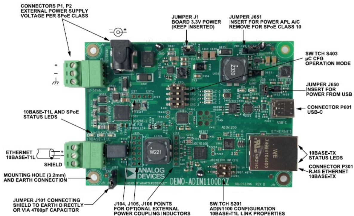
Figure 2. Board Connectors and Controls
