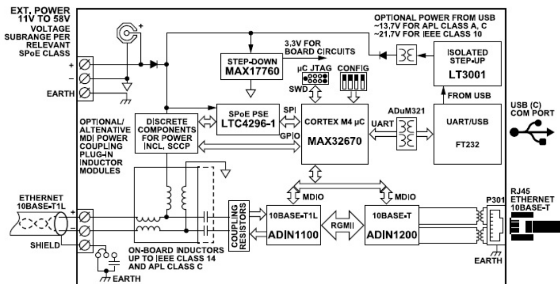
Figure 3. Simplified Block Diagram
