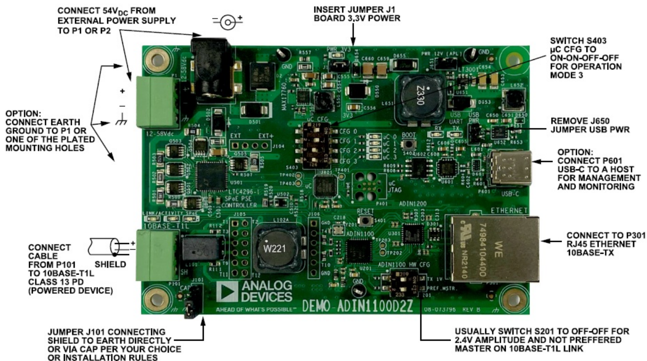
Figure 6. Board Setup for SPoE Class 13
