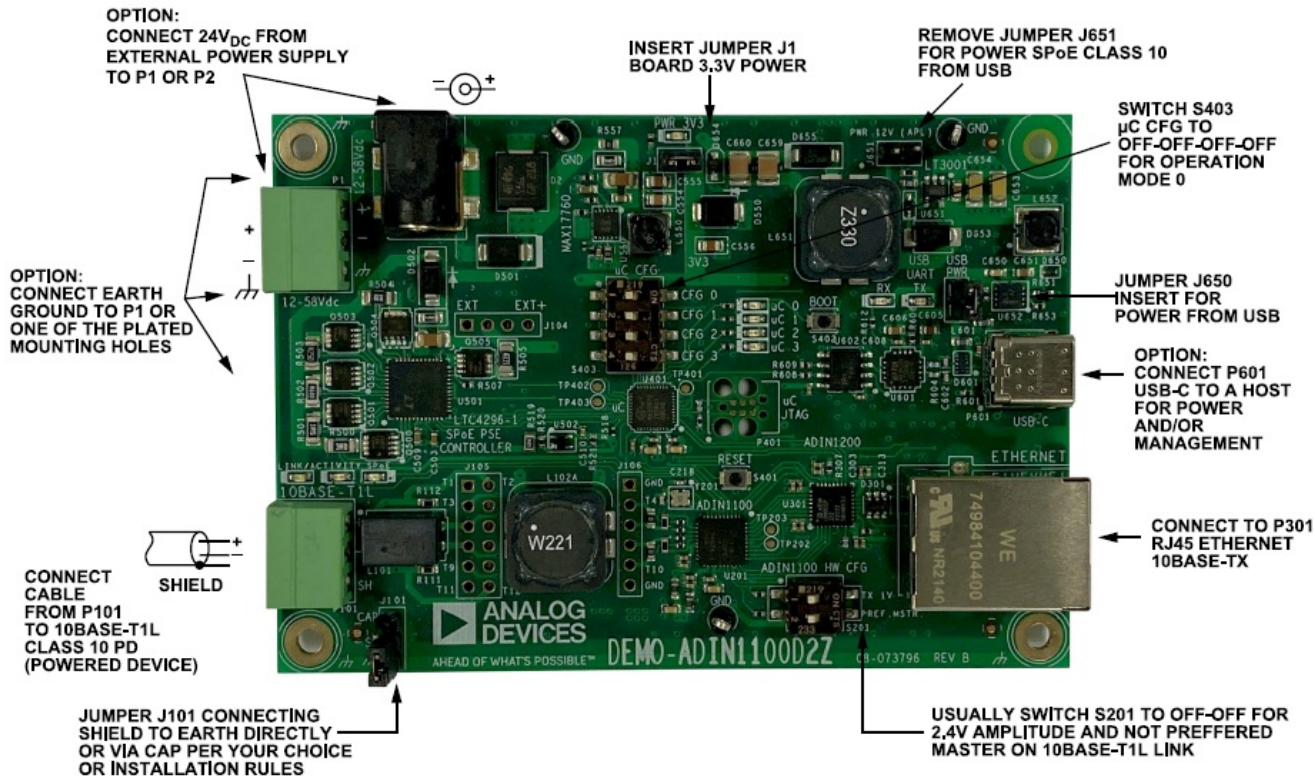
Figure 4. Board Setup for SPoE Class 10
