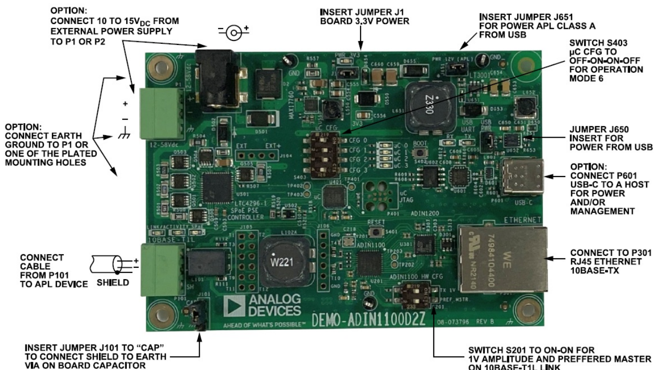
Figure 11. Board Setup for APL Class A
