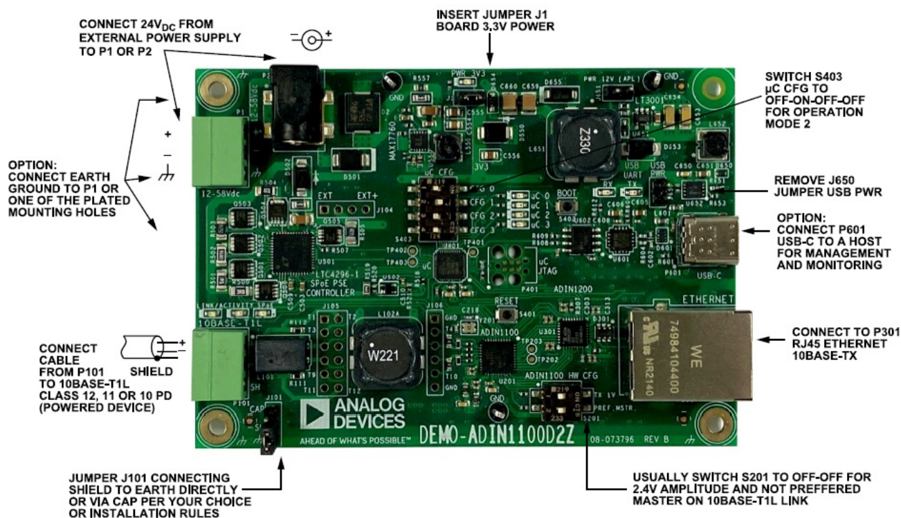
Figure 5. Board Setup for SPoE Class 12
