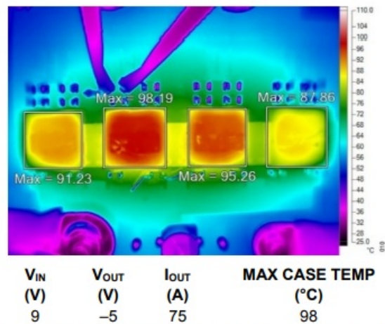
Figure 10. Thermal Capture with 400LFM Airflow, T_A = 25^\circ C
