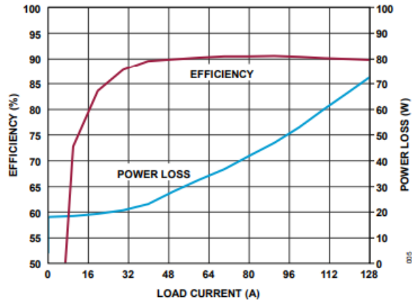
Figure 5. Sourcing Current Efficiency vs. Power Loss
