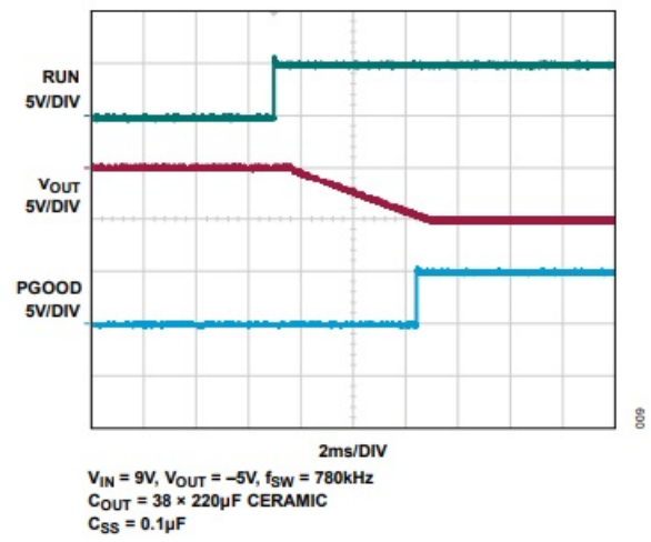
Figure 9. Startup with No Load
