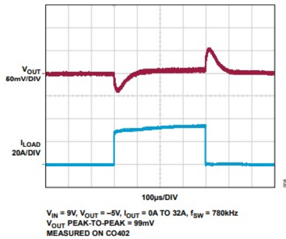
Figure 8. Load Transient Response
