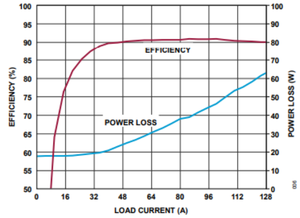
Figure 6. Sinking Current Efficiency vs. Power Loss
