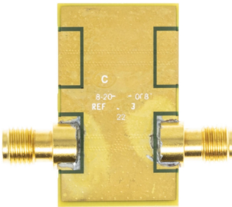
Figure 2. ADL8107-EVALZ Secondary Side
