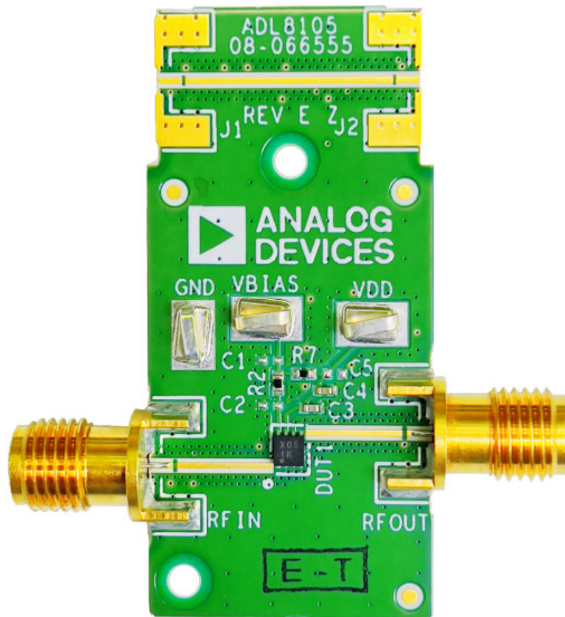
Figure 1. ADL8105-EVALZ Primary Side
