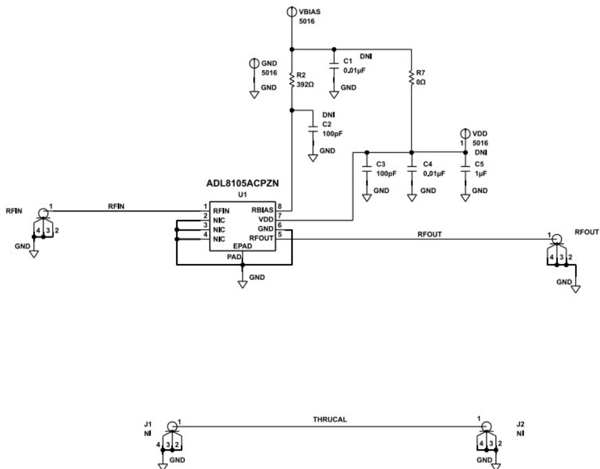
Figure 4. ADL8105-EVALZ Schematic
