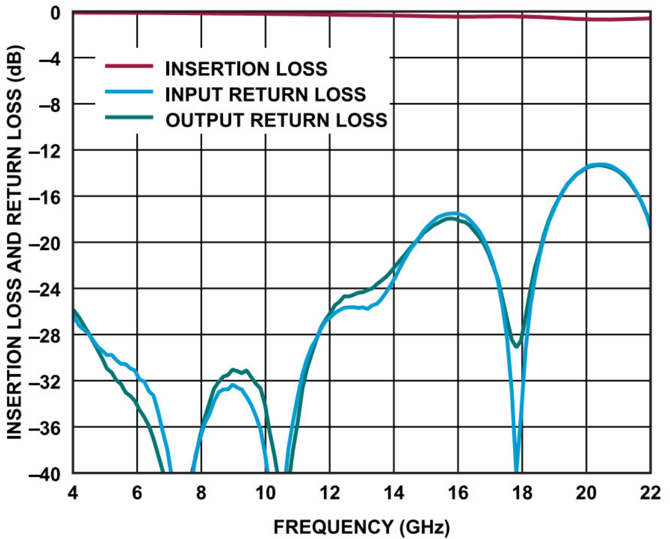
Figure 3. Insertion Loss and Return Loss of the Through Calibration Path
