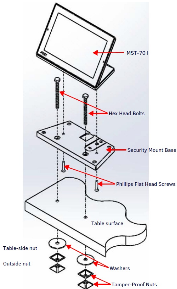
FIG. 2 INSTALLATION PROCEDURE, EXPLODED DIAGRAM
