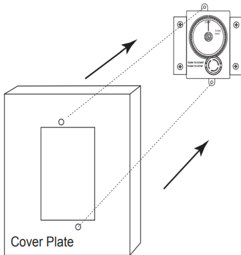
Fig. 5 Installing cover plate.
