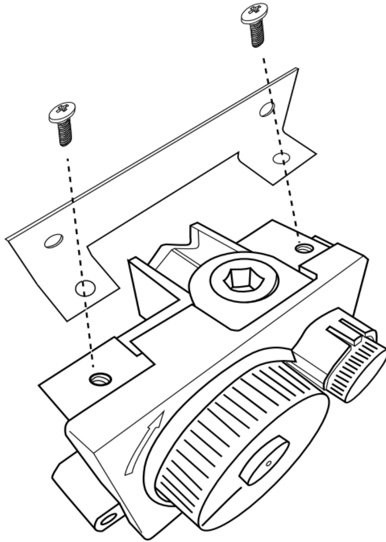
Fig. 1 Installing mounting brackets to ESTOP gas timer.
