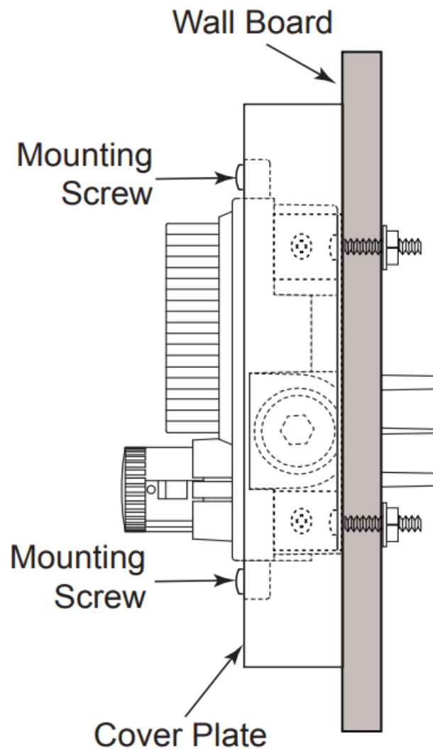
Fig. 6 Side view of ESTOP mounted into wall.
