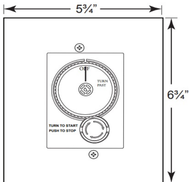
Fig.7 Cover plate outer dimensions.
