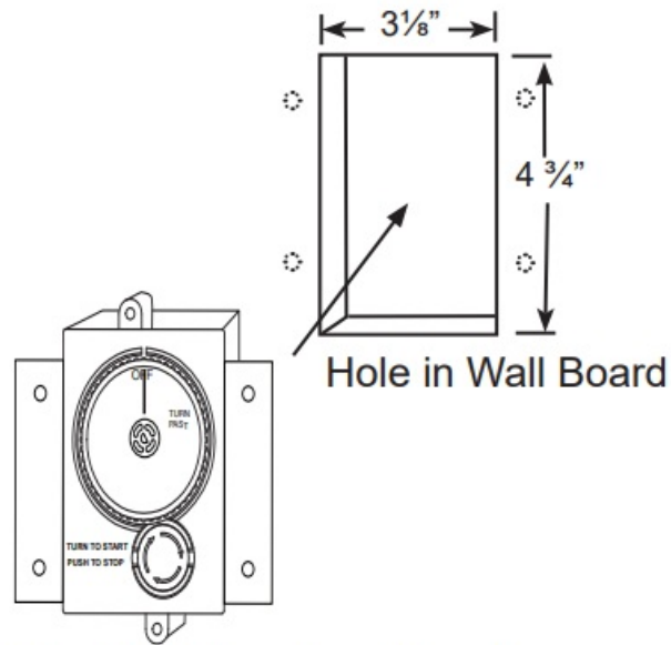
Fig. 3 Installing ESTOP gas timer into wall.
