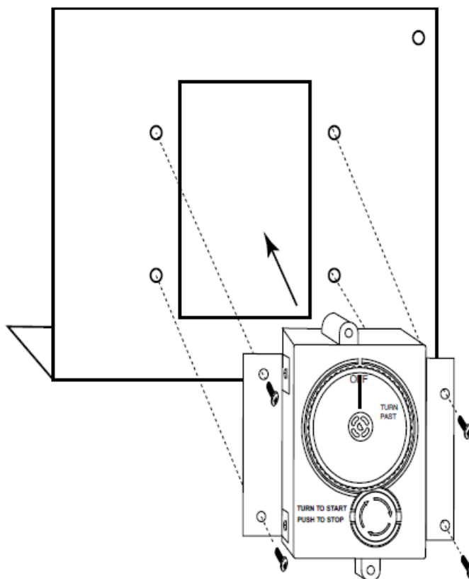
Fig. 3 Shows ESTOP mounted into paver bracket.
