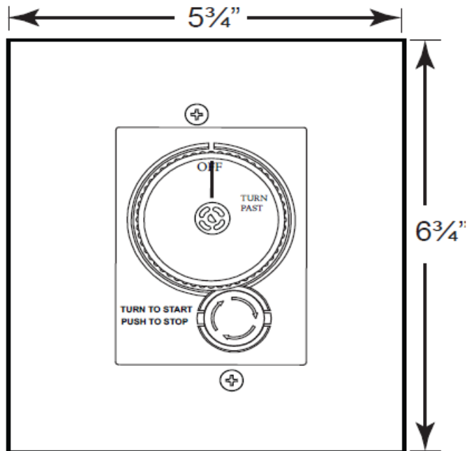
Fig.8 Cover plate outer dimensions.
