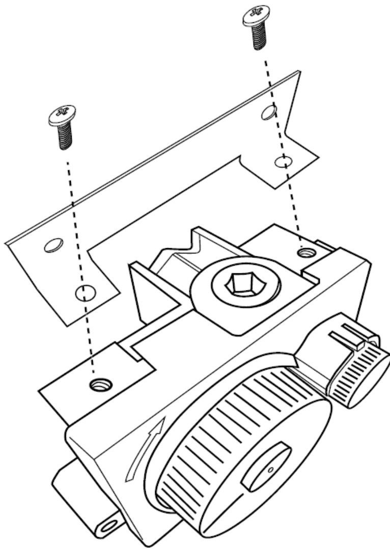
Fig. 1 Installing mounting brackets to ESTOP gas timer.
