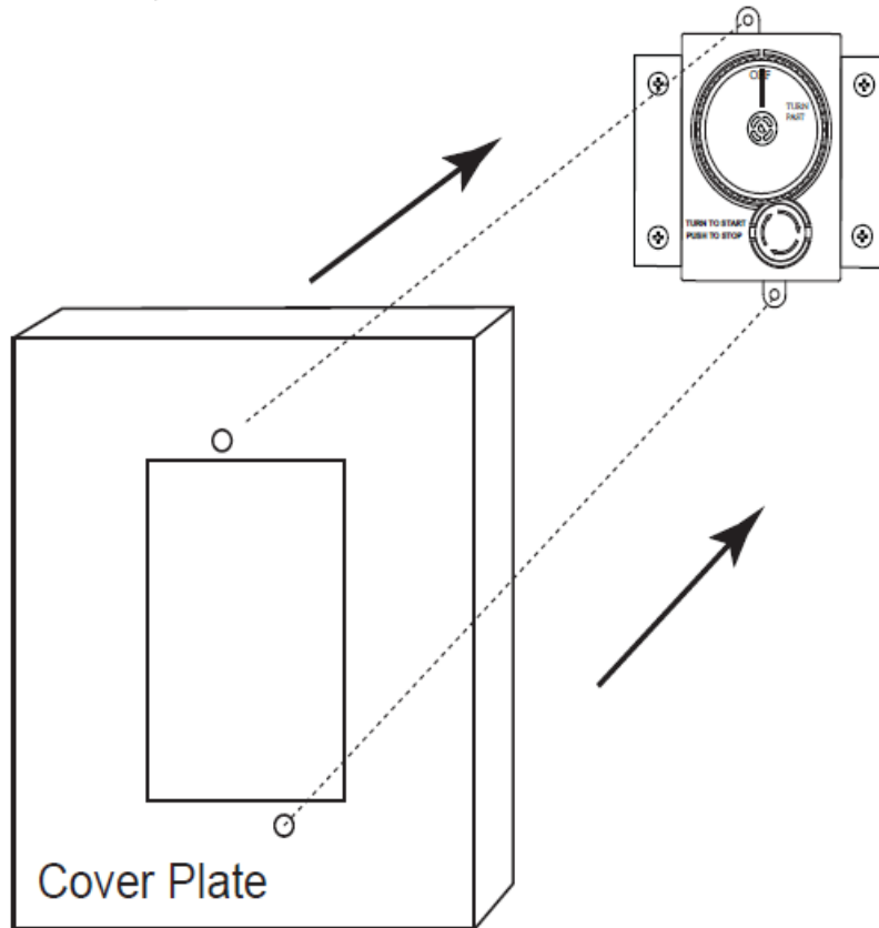
Fig. 7 Installing cover plate.
