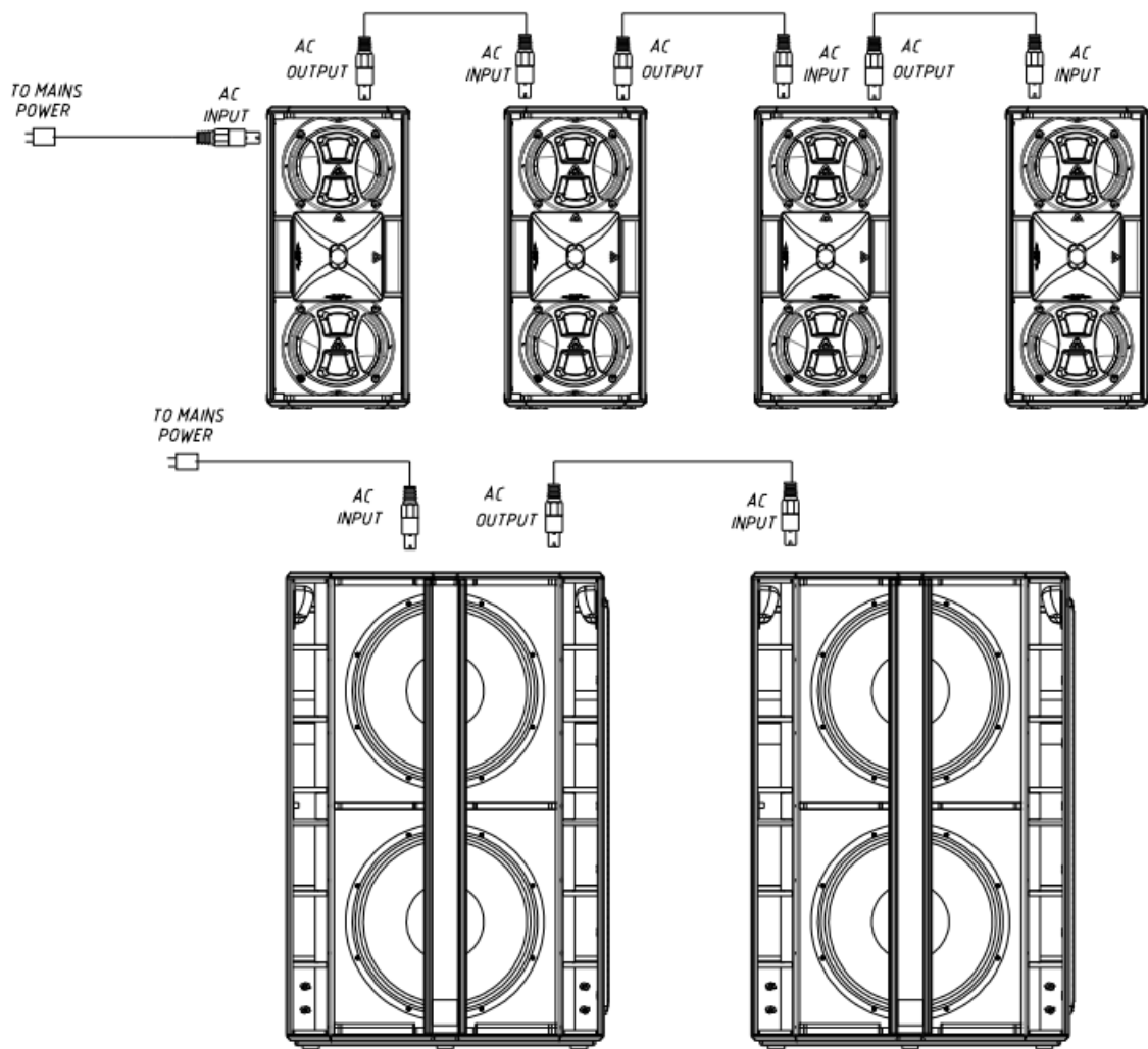
Fig. 11. Parallel connection for the X102FD and X218WFD (mains). Do not connect more than four units of X102FD or two units of X218WFD using the AC Mains link connector.
