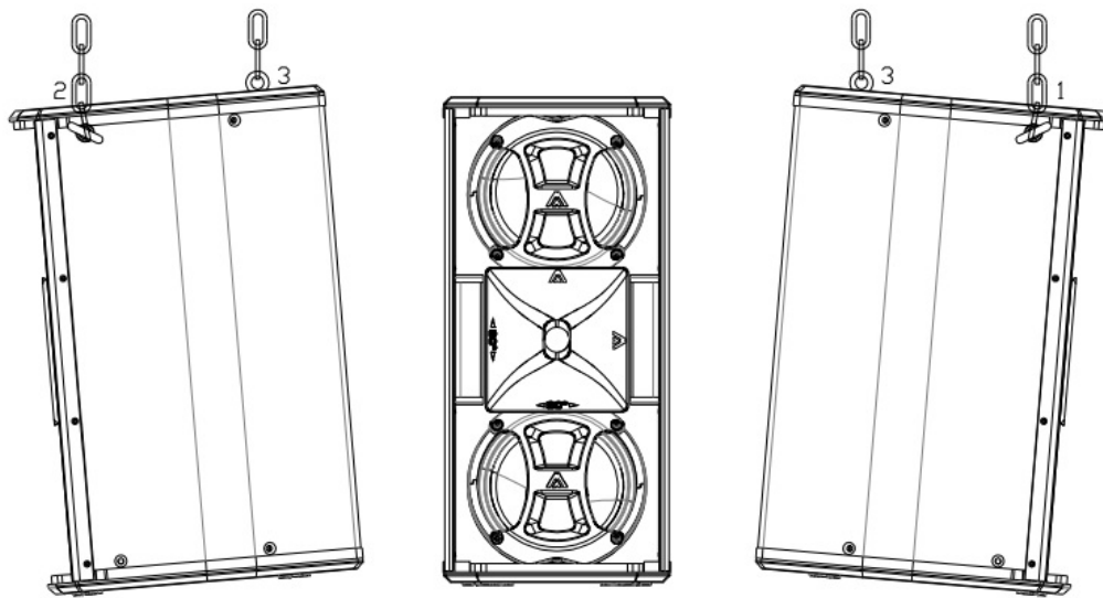
Fig. 18. X102FD vertical flying
