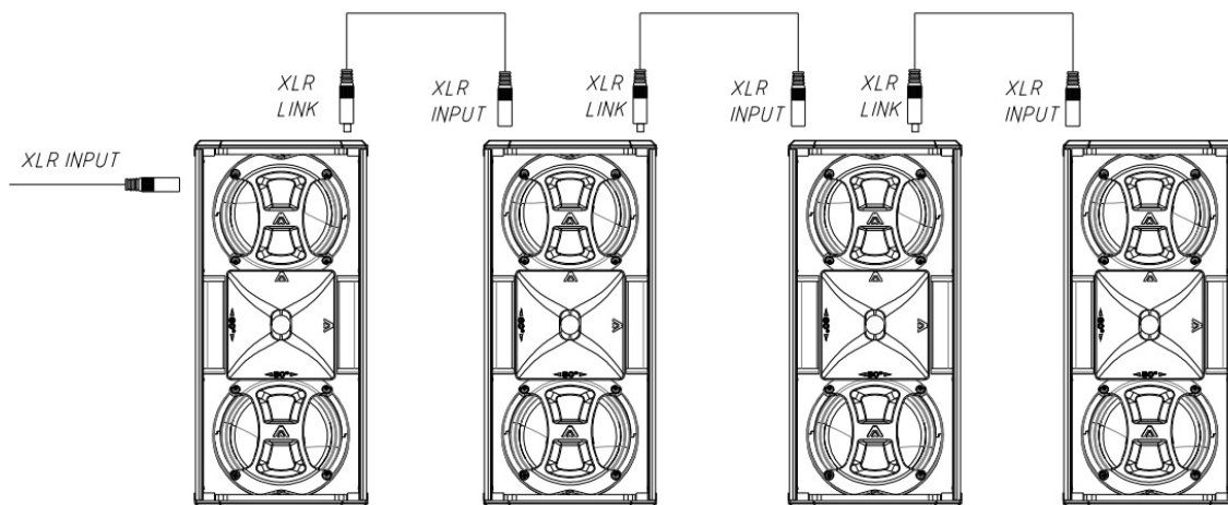
Fig. 7. Parallel connection for the X102FD (signal)
