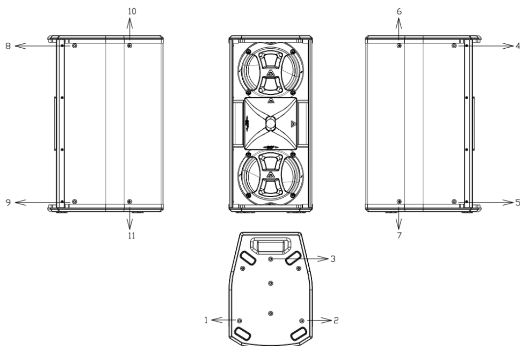
Fig. 17. X102FD horizontal and vertical flying points
