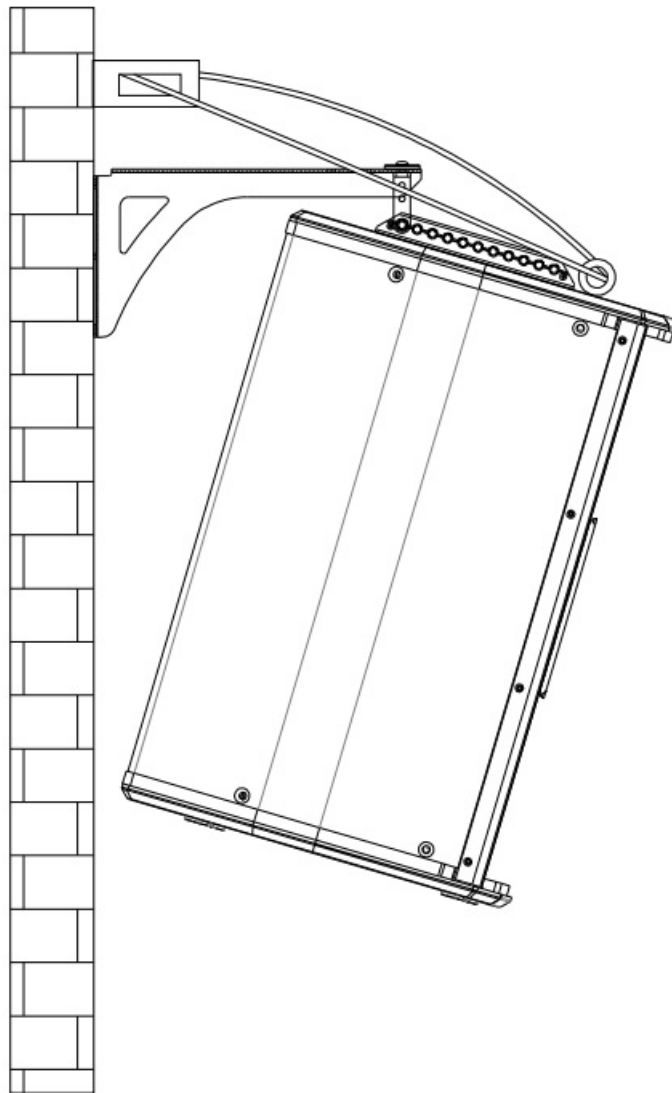
Fig. 22. Flying of one unit X102FD with SPWHR
