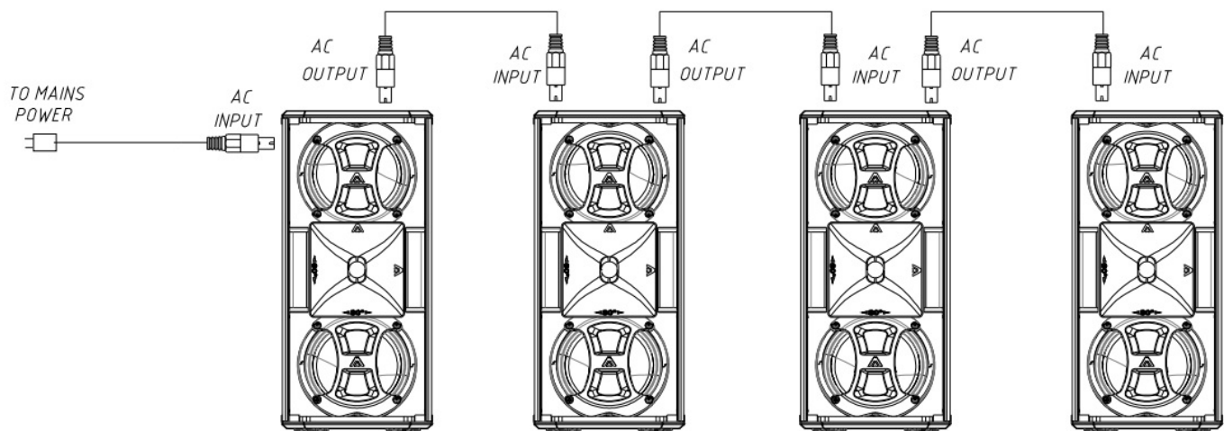
Fig. 8. Parallel connection for the X102FD (mains). You can link up to four units
