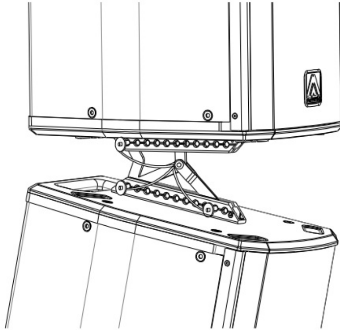
Fig. 20. Flying of two units X102FD with HR-L102
