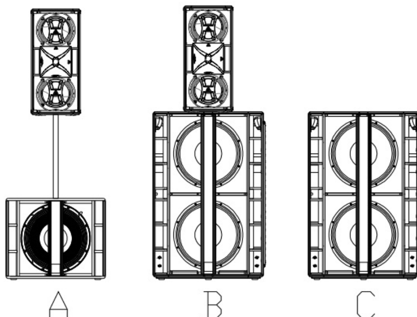
Fig. 15. X102FD with subwoofer (A: with pole, B: stacked, C: flown)
