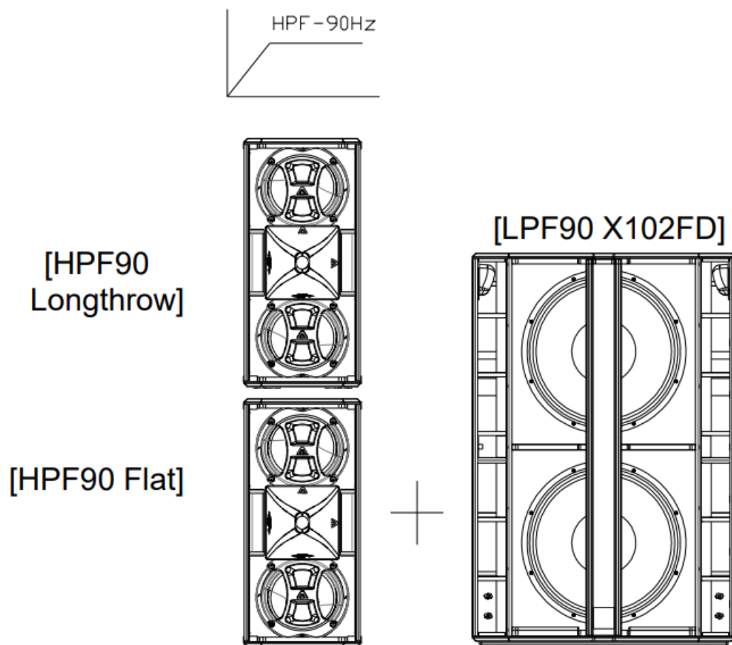
Fig. 5. Preset [HPF90 Longthrow] configuration
