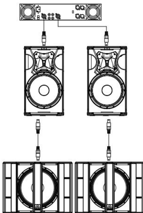
Fig. 4. Passive configuration with subwoofer
