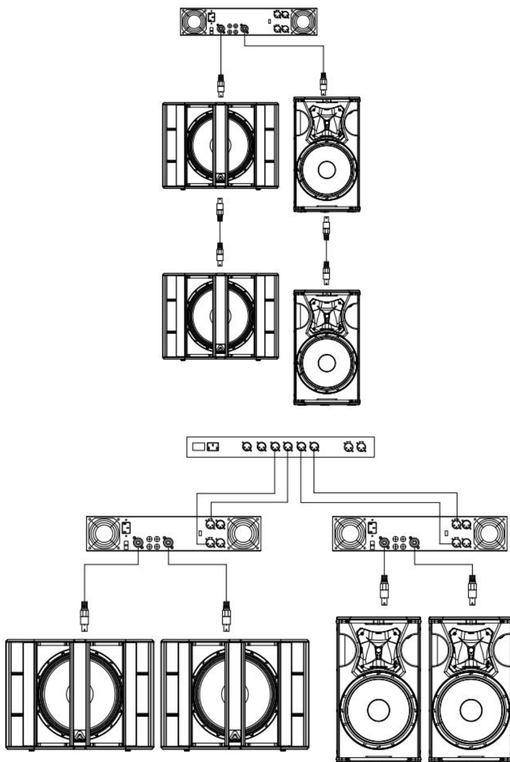
Fig. 6. Bi-amplified with subwoofer configuration (option 2)
