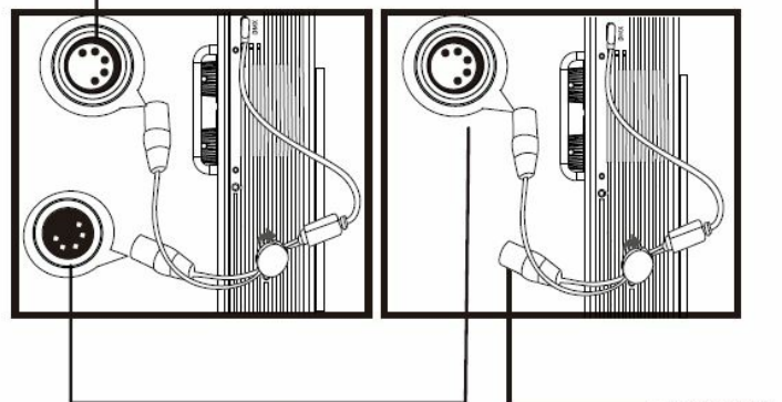
Daisy chaining multiple lights using DMX
