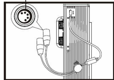
Connecting DMX to only one light
