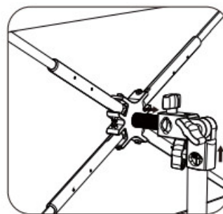
Bracket
