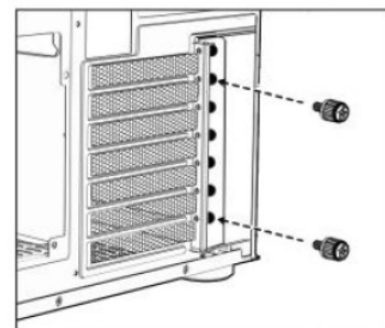
B Screw #6-32 x 7 For PCI
