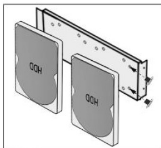
A Screw #6-32_5mm x 8 For HDD
