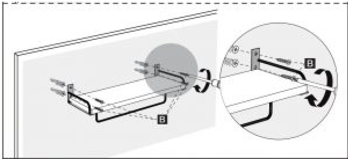
Step 1C For Solid Concrete and Concrete Block Walls
