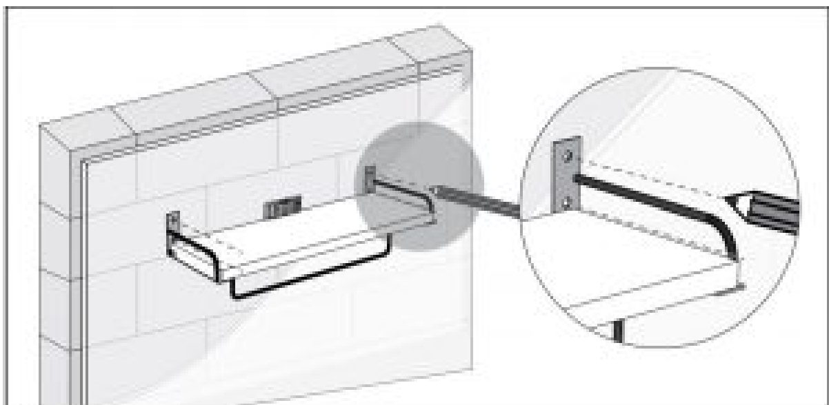
Step 1C For Solid Concrete and Concrete Block Walls
