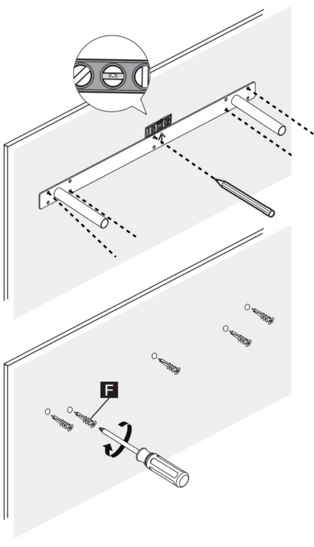
Step 1C For Solid Concrete and Concrete Block Walls
