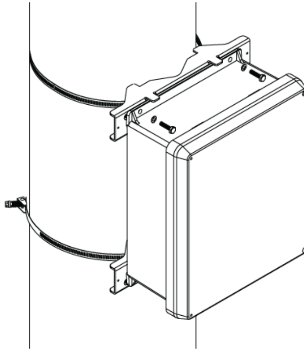
Fig. 7a 5" (127mm) square pole
