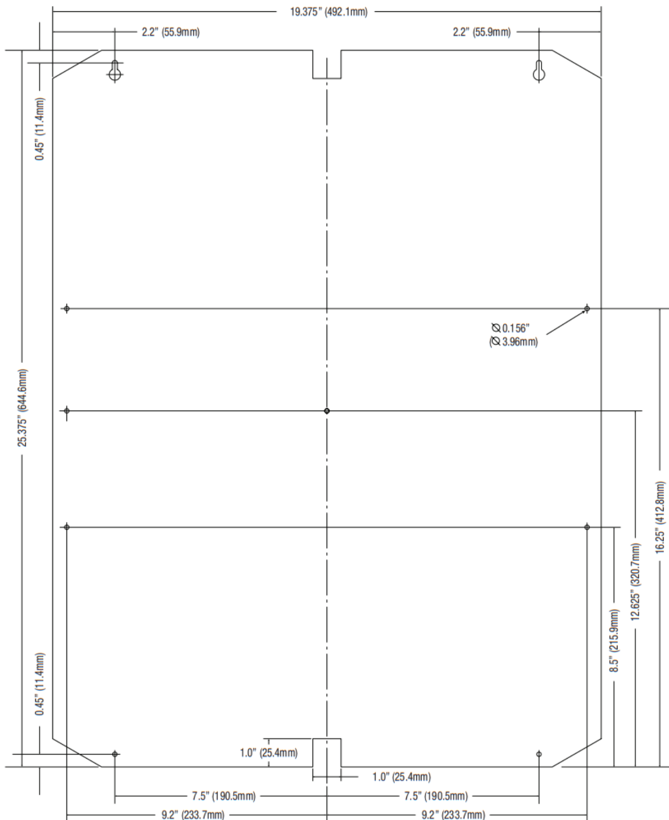
Trove2KS2 Enclosure Dimensions (H x W x D approximate): 27.25" x 21.75" x 6.5" (692.2mm x 552.5mm x 165.1mm)
