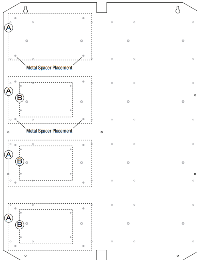
Fig. 2 - Trove2Z2/TZ2 Configurations
