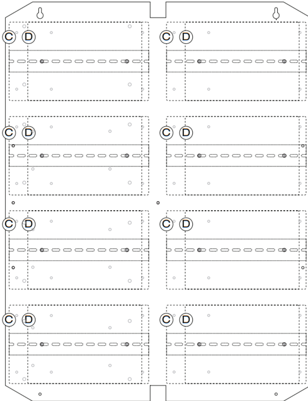
Fig. 3 - Trove2Z2/TZ2 Configurations
