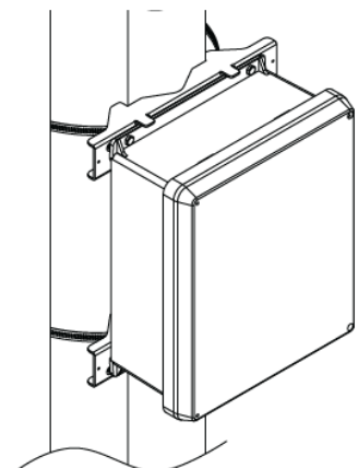
Fig. 8a 5" (127mm) square pole
