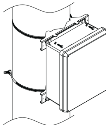
Fig. 8 2" to 8" (50.8mm to 203.2mm) diameter round pole
