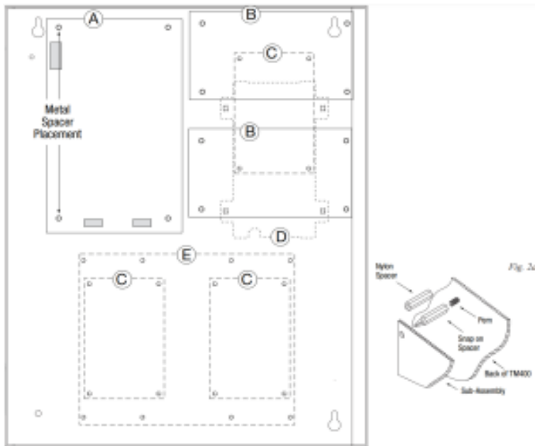
Fig. 2 – Altronix and Mercury configurations
