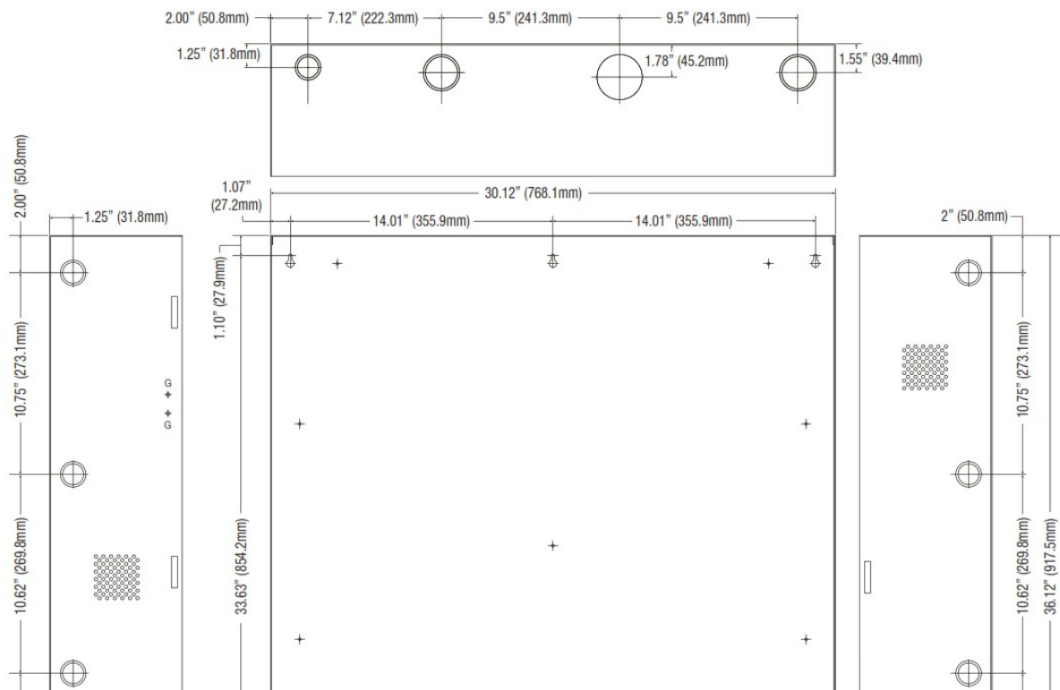
Trove3 Enclosure Dimensions (H x W x D approximate): 36.12" x 30.125" x 7.06" (917.5mm x 768.1mm x 179.3mm)
