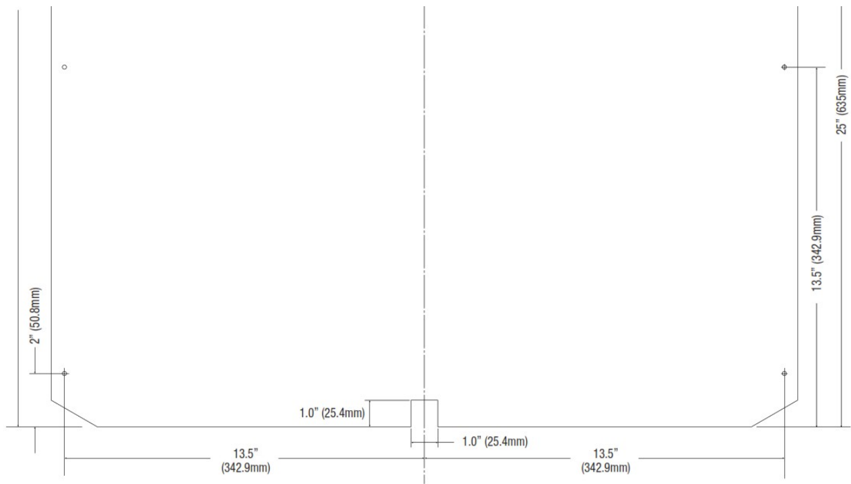
Trove3 Enclosure Dimensions (H x W x D approximate): 36.12" x 30.125" x 7.06" (917.5mm x 768.1mm x 179.3mm)
