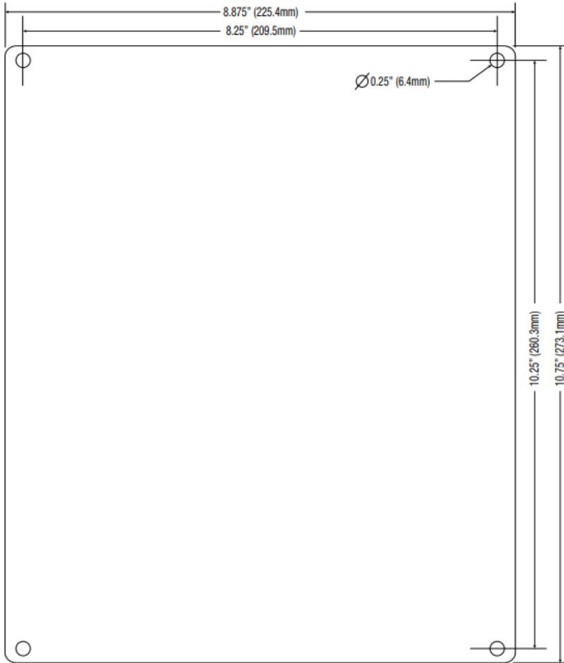
NetWaySP4LPL Mechanical Drawing and Dimensions (H x W x D approx.): 10.75" x 8.875" x 2.375" (273.1mm x 225.4mm x 60.3mm)
