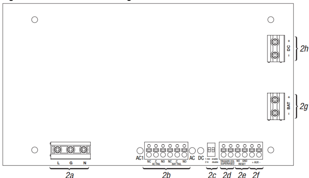
Fig. 2 – eFlow104NB Board Configuration
