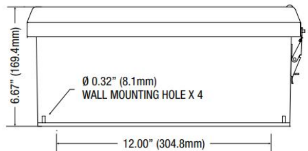
END VIEW
