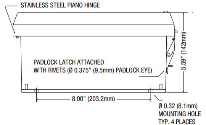
END VIEW
