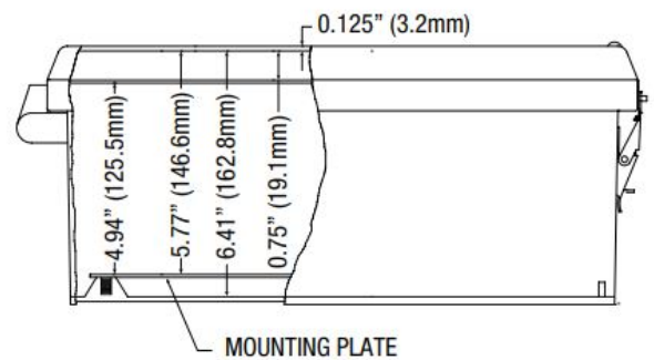
END VIEW
