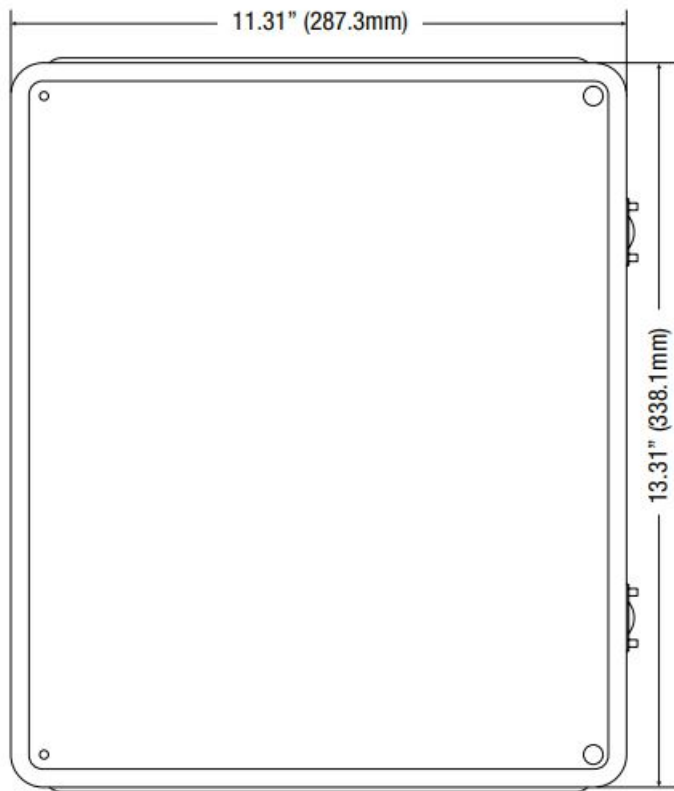
FRONT VIEW COVER REMOVED
