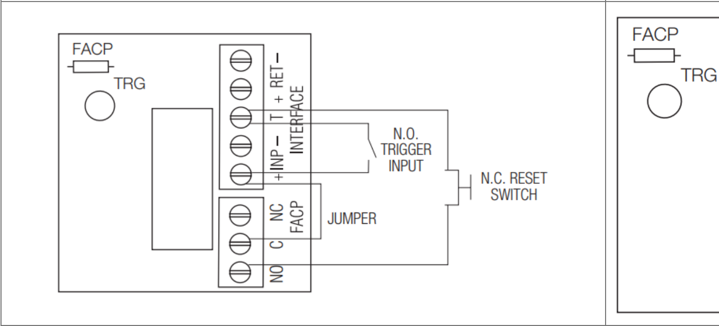
Fig. 7 Normally Open FACP Latching trigger input with reset (This output has not been evaluated by UL): Fig. 8 Normally C
