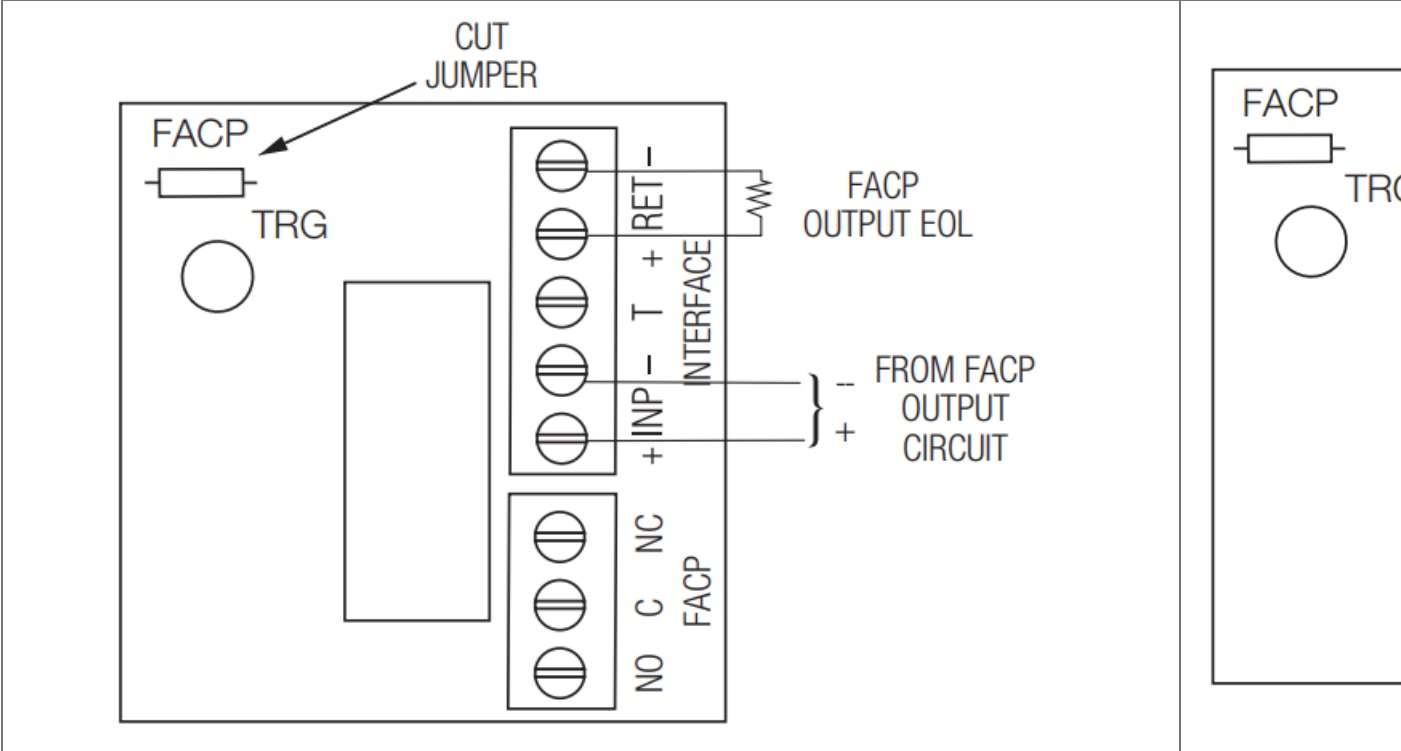
Fig. 7 Normally Open FACP Latching trigger input with reset (This output has not been evaluated by UL): Fig. 8 Normally C
