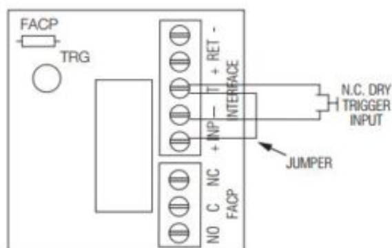
Fig. 10 Normally Closed: Non-Latching FACP trigger input:
