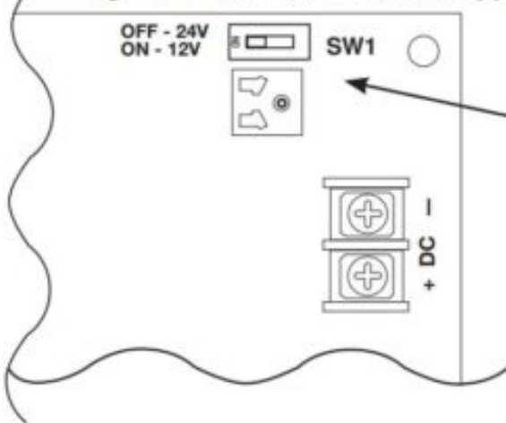
Fig. 1a - Maximal3D Power Supply Board
