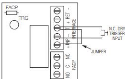
Fig. 10 Normally Closed: Non-Latching FACP trigger input:
