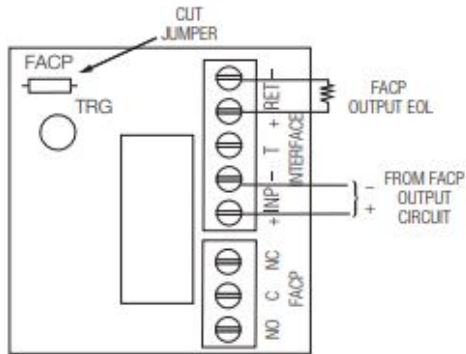
Fig. 9 Normally Open: Non-Latching FACP trigger input:
