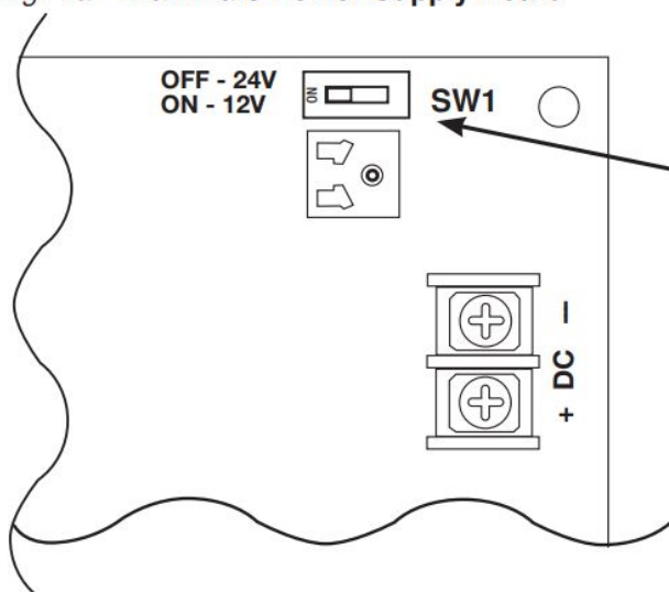
Fig. 1a - Maximal3 Power Supply Board
