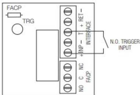
Fig. 9 Normally Open: Non-Latching FACP trigger input:
