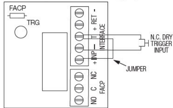
Fig. 14 Normally Closed - Non-Latching FACP trigger input:
