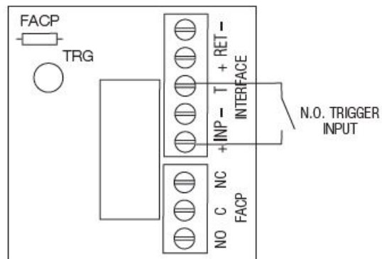
Fig. 12 Normally Open - Non-Latching FACP trigger input:
