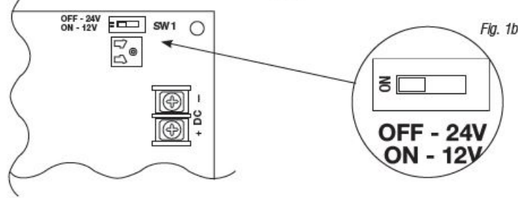
Fig. 1a - Maximal11 and Maximal33 Power Supply Board
