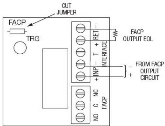
Fig. 12 Normally Open - Non-Latching FACP trigger input:
