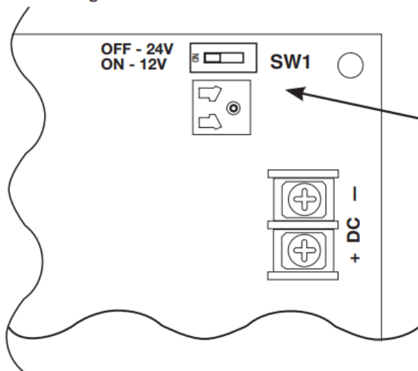
Fig. 1a - AL400XB2V / AL600XB220 Power Supply Board
