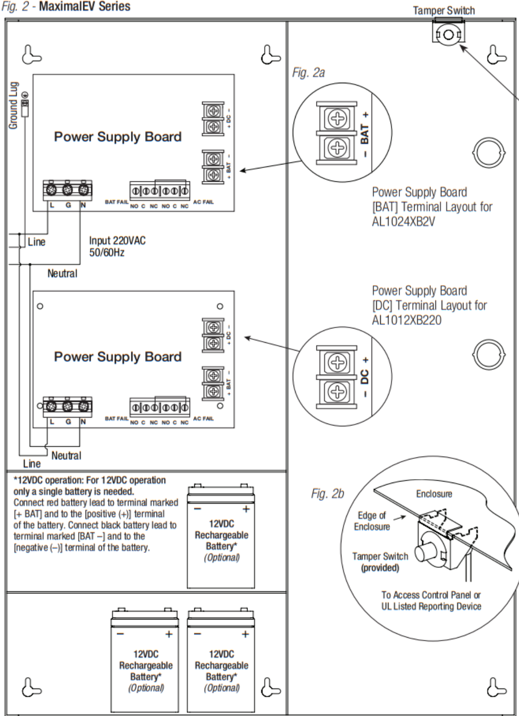
Fig. 2 - MaximalEV Series
