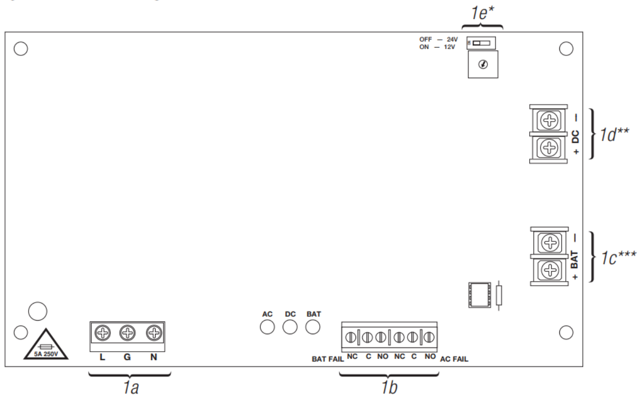
Fig. 1 - ULXB Board Configuration
