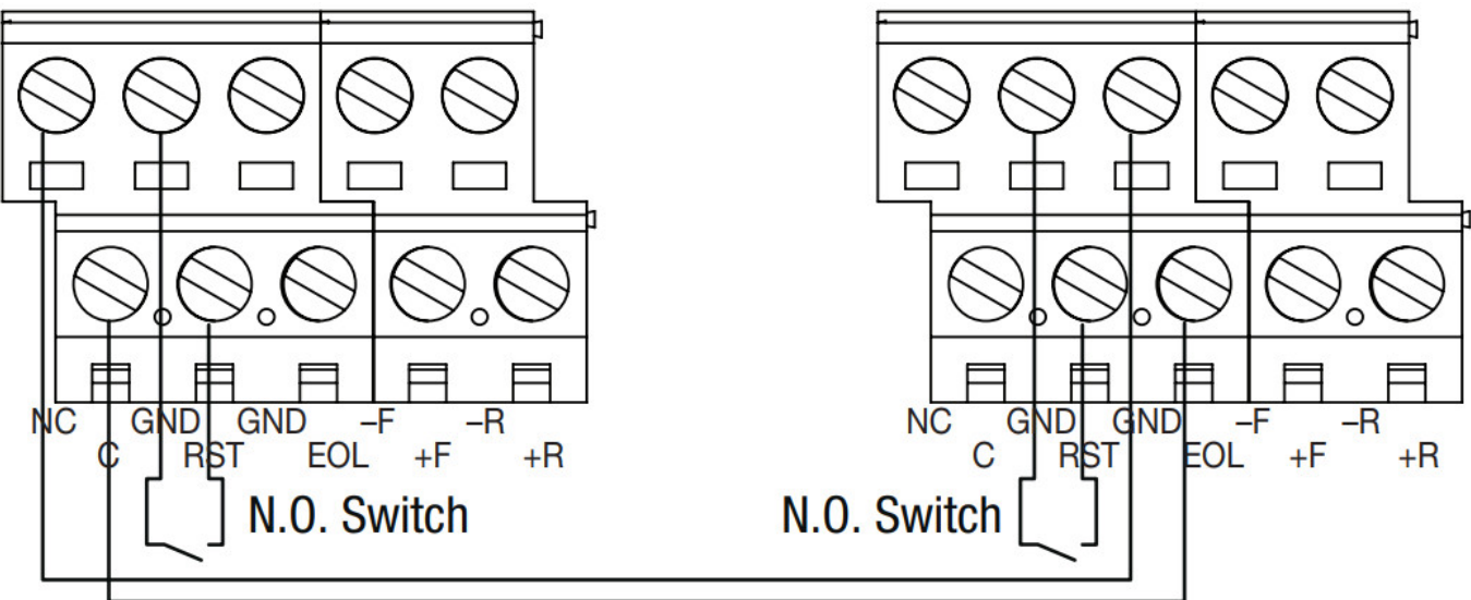
Fig. 10 – Polarity reversal input from FACP signaling circuit output (polarity is referenced in alarm condition). Non-Latching.
