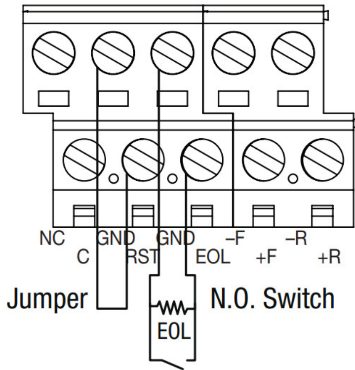
Fig. 15 – Normally Open trigger input (Latching).
