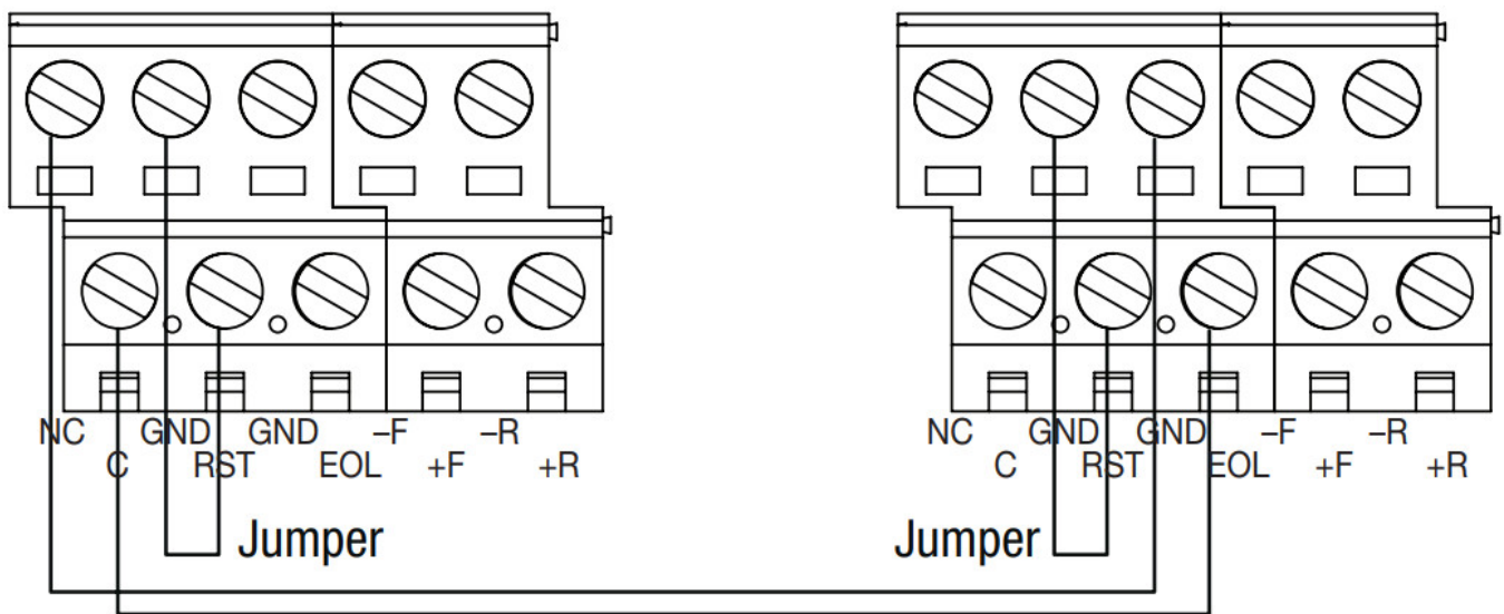
Fig. 9 – Daisy-chaining one or more ACMS12 units.
