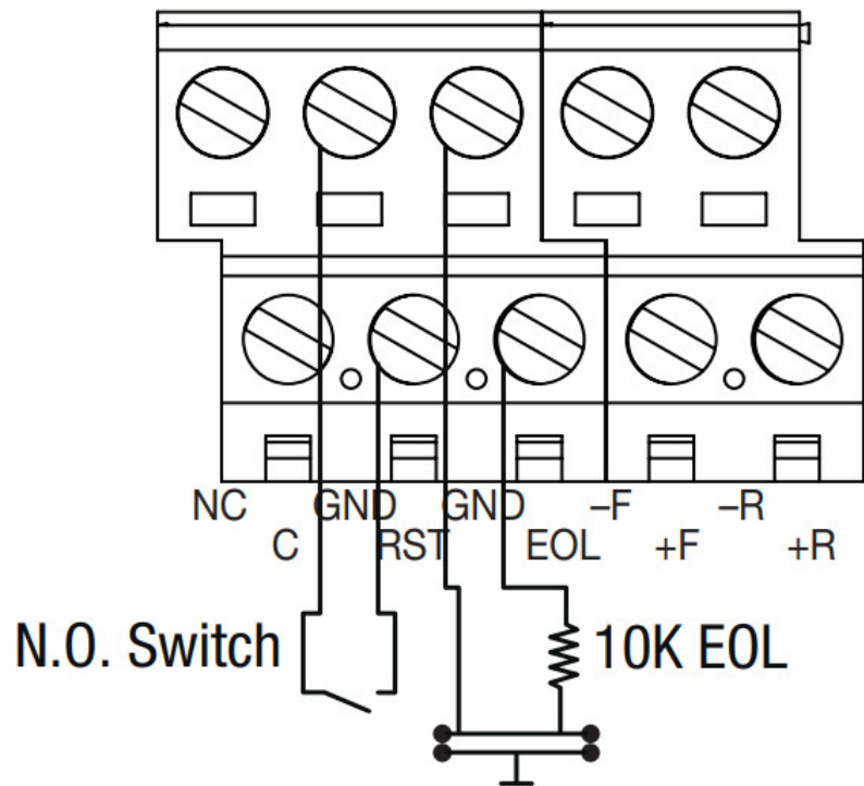
Fig. 15 – Normally Open trigger input (Latching).
