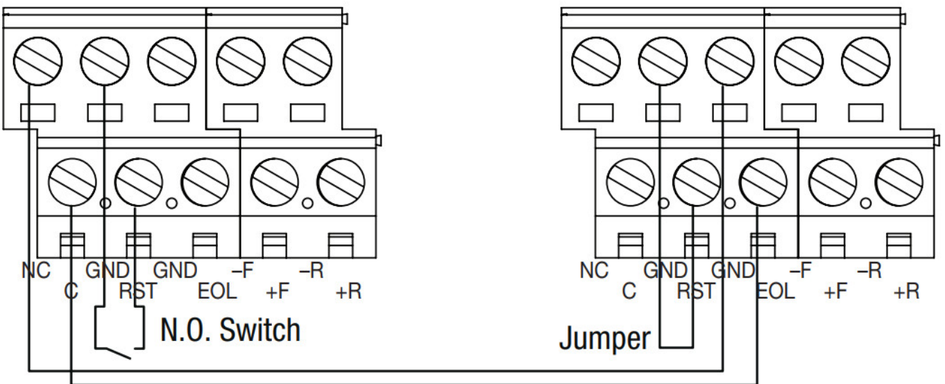
Fig. 10 – Daisy chaining one or more ACMS12 units.
