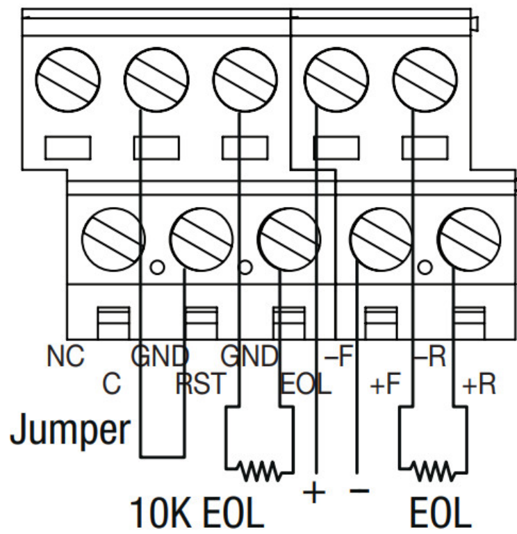
Fig. 11 – Polarity reversal input from FACP signaling circuit output (polarity is referenced in alarm condition). Latching.
