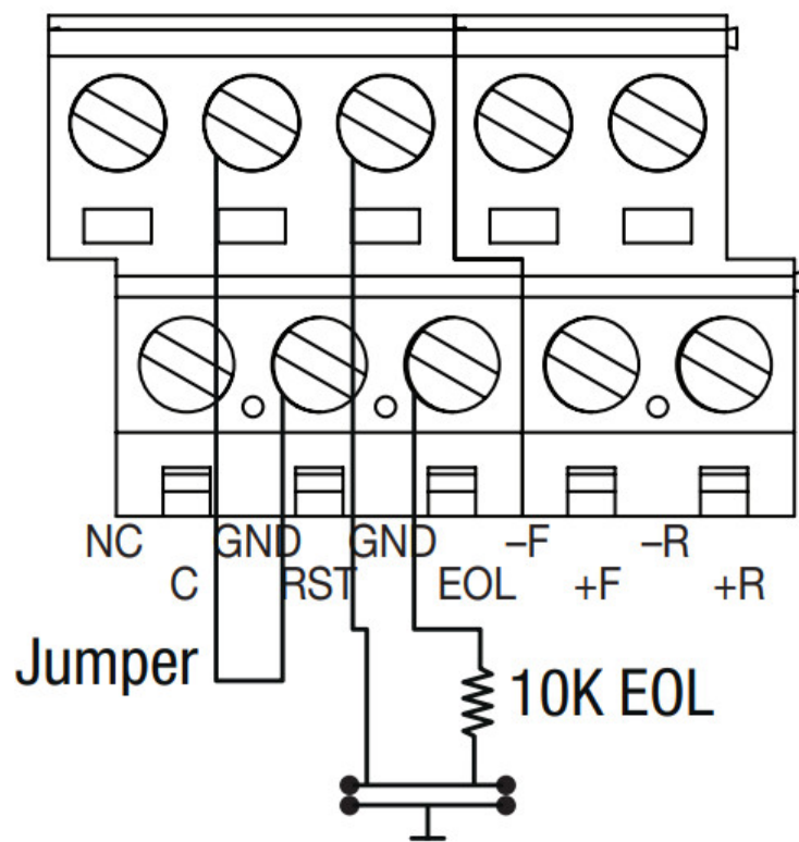
Fig. 13 – Normally Closed trigger input (Latching).
