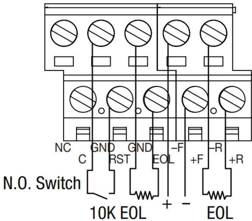
Fig. 12 – Normally Closed trigger input (Non-Latching).
