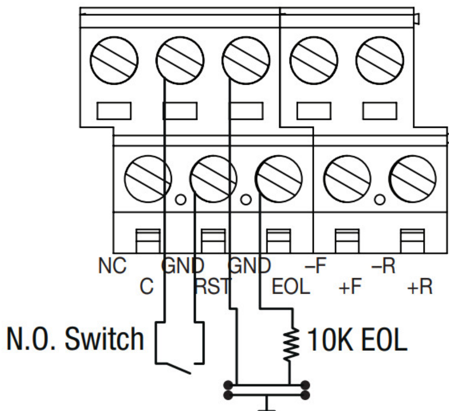
Fig. 14 – Normally Open trigger input (Non-Latching).
