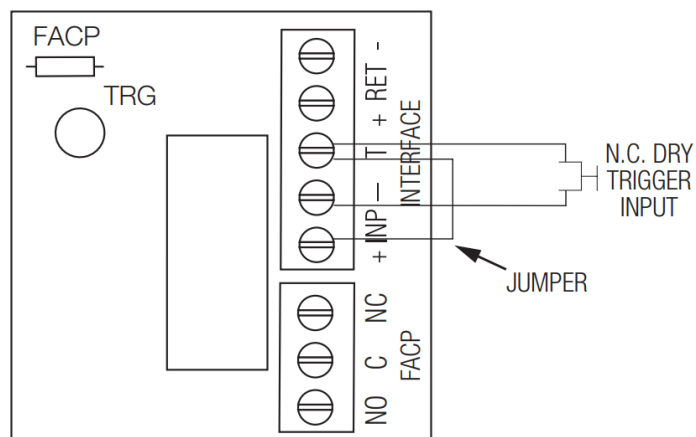
Fig. 7 Normally Closed: Non-Latching FACP trigger input:
