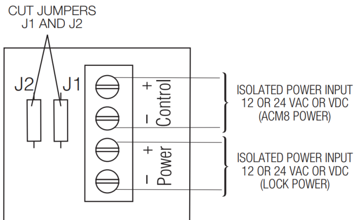
Fig. 3 Optional hook-up using two (2) isolated power supply inputs:
