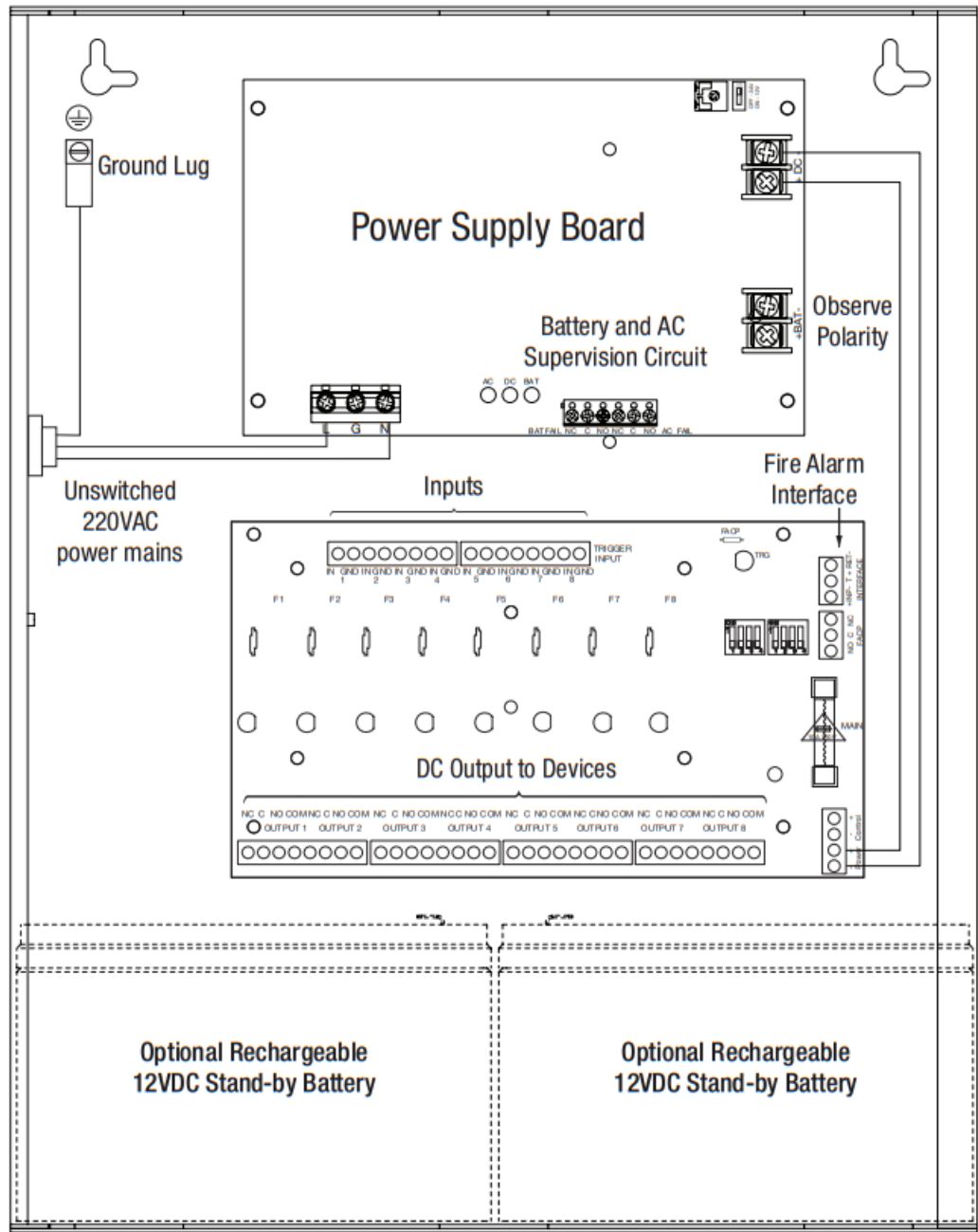
Fig. 2 – ACMCB220 Series Configuration
