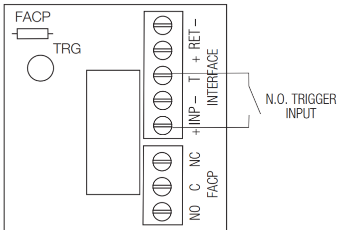
Fig. 6 Normally Open FACP Latching trigger input with reset (This output has not been evaluated by UL):
