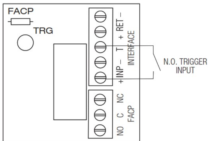
Fig. 5 Normally Open FACP Latching trigger input with reset (This output has not been evaluated by UL):
