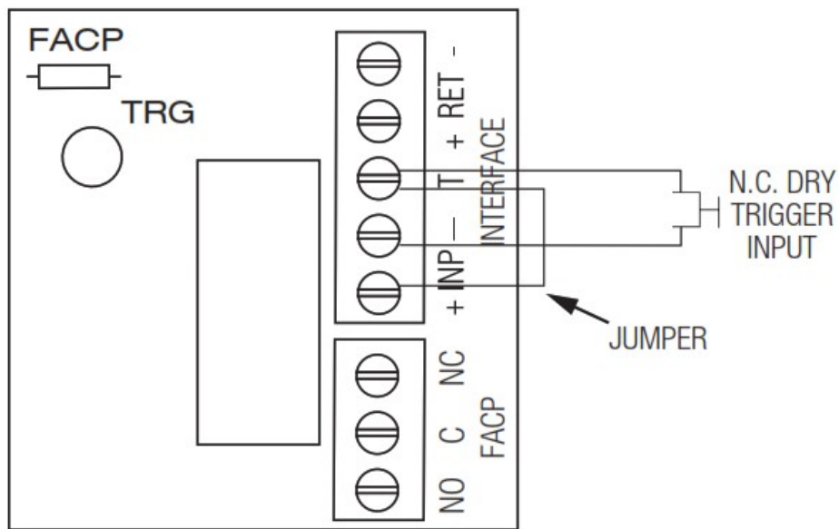
Fig. 7 Normally Closed: Latching FACP trigger input with reset (This output has not been evaluated by UL):
