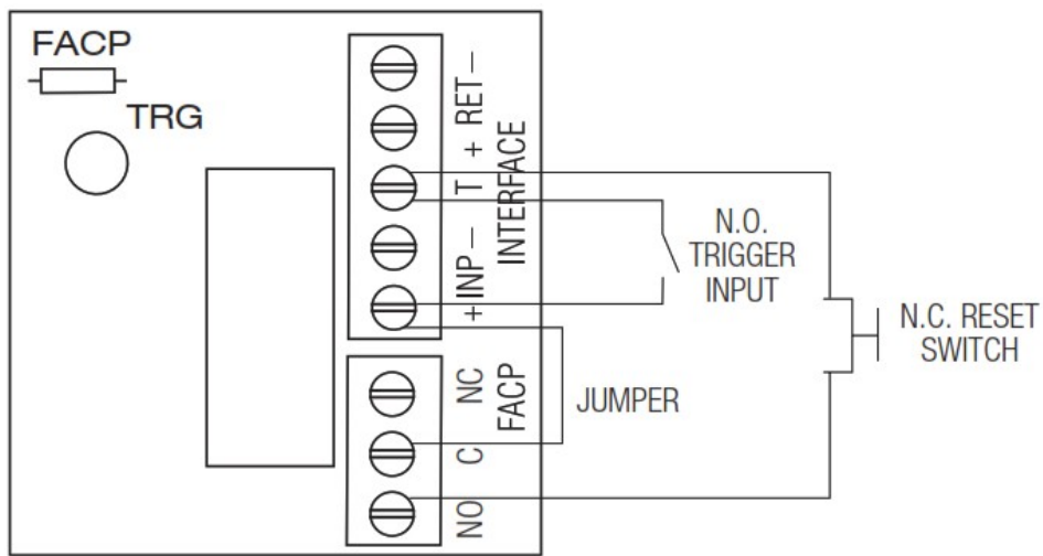
Fig. 6 Normally Closed: Non-Latching FACP trigger input:
