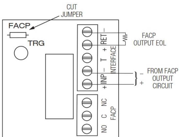
Fig. 4 Normally Open: Non-Latching FACP trigger input:
