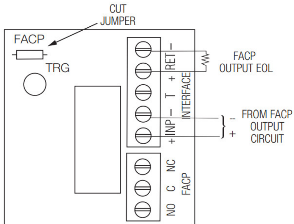
Fig. 4 Normally Open: Non-Latching FACP trigger input:
