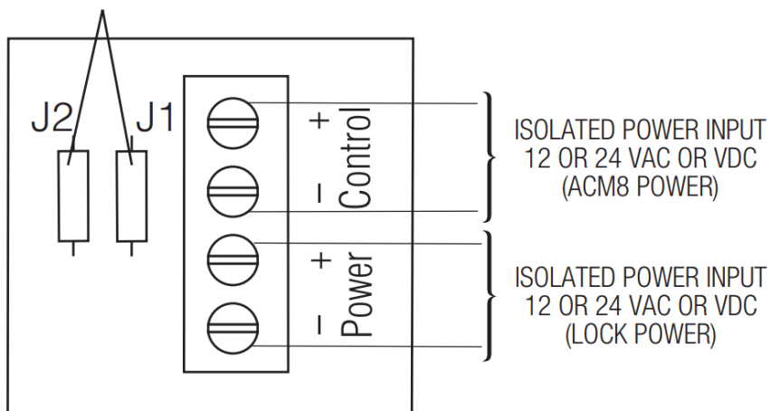
Fig. 4 Polarity reversal input from FACP signaling circuit output (polarity is referenced in alarm condition):
