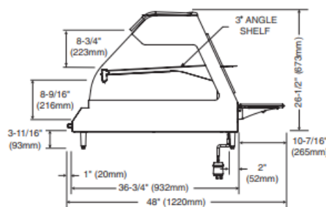
ED2-2S PROFILE
