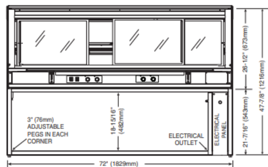
ED2SYS-72/2S
