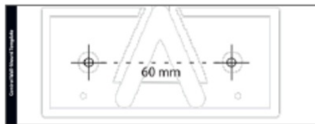
Horizontal Mount
